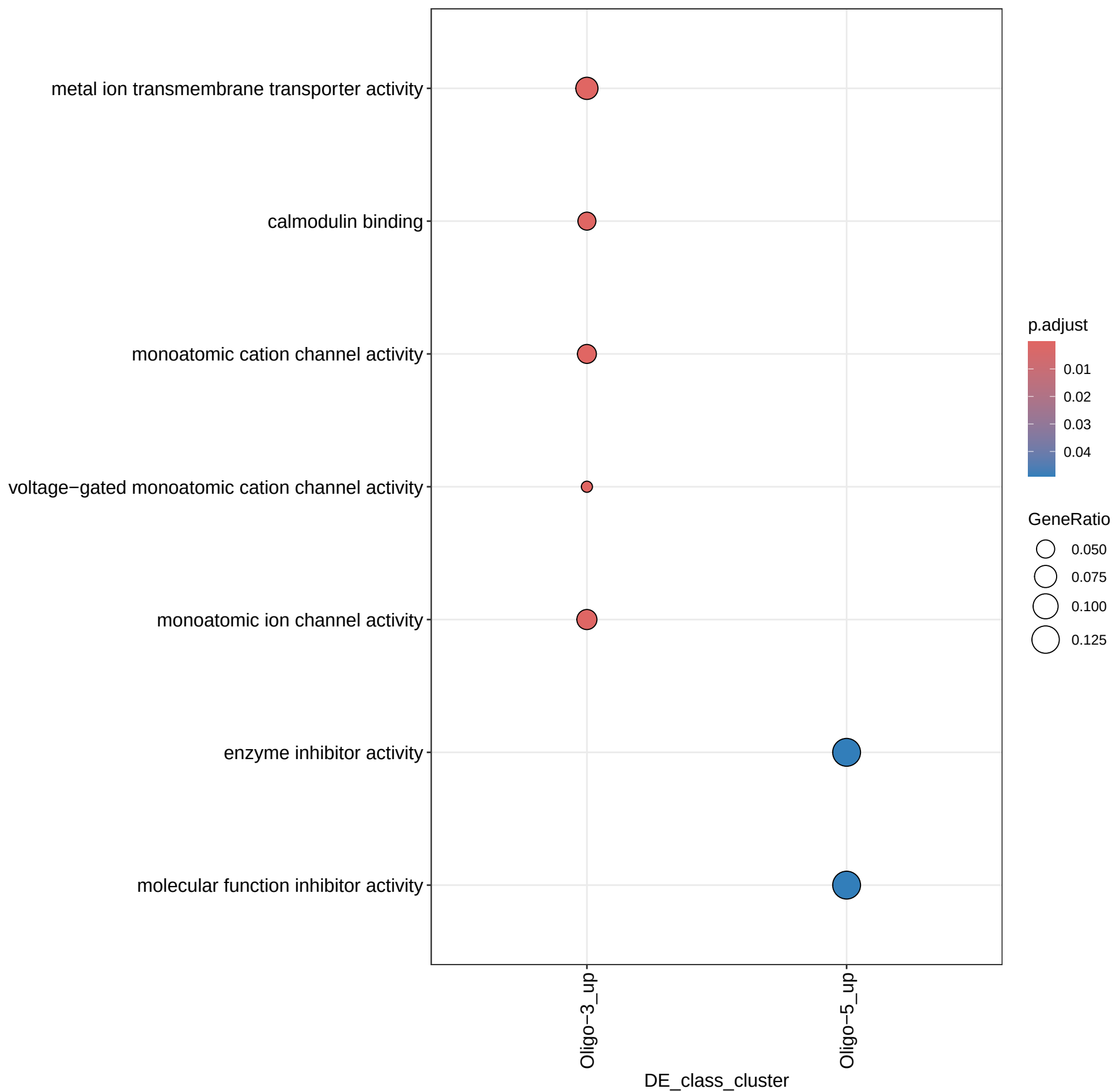
GO Enrichment:MF – Oligo (5+ genes)
