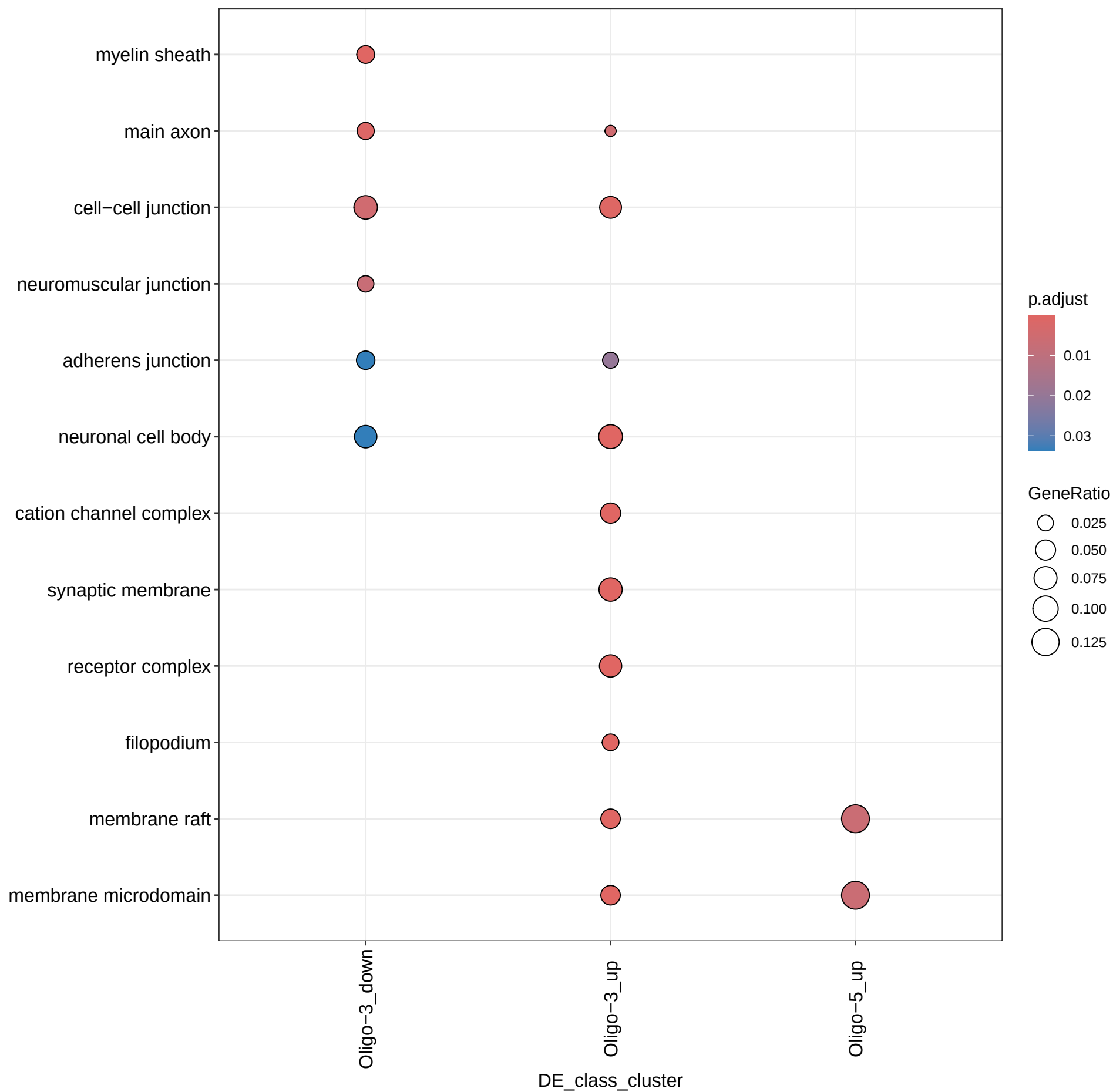
GO Enrichment:CC – Oligo (5+ genes)
