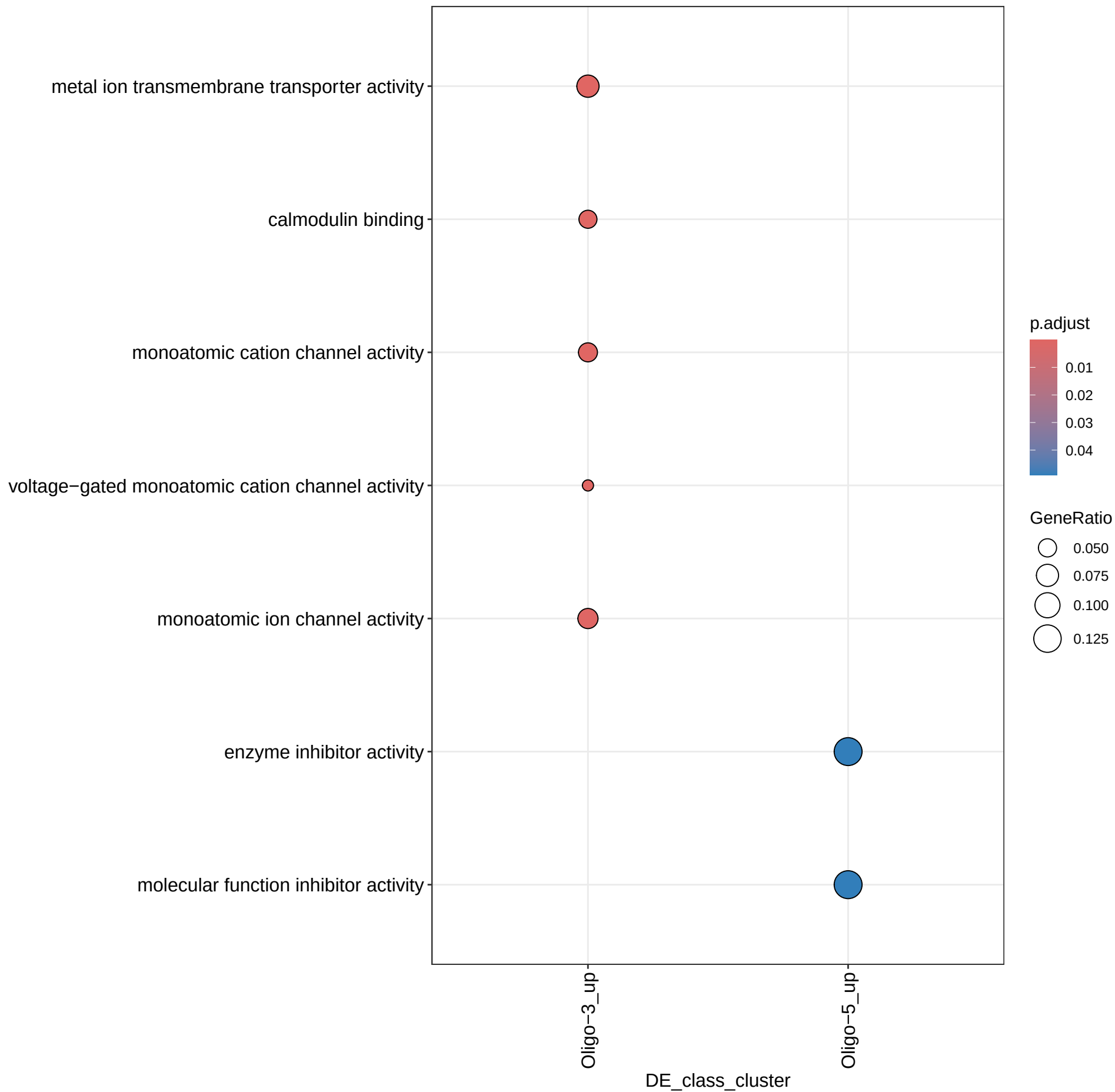
GO Enrichment:MF – Oligo (5+ genes)
