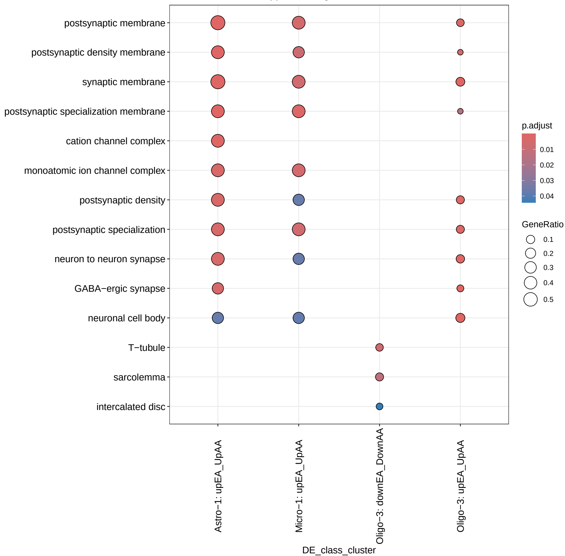
GO Enrichment: CC opposite, 2+ genes
