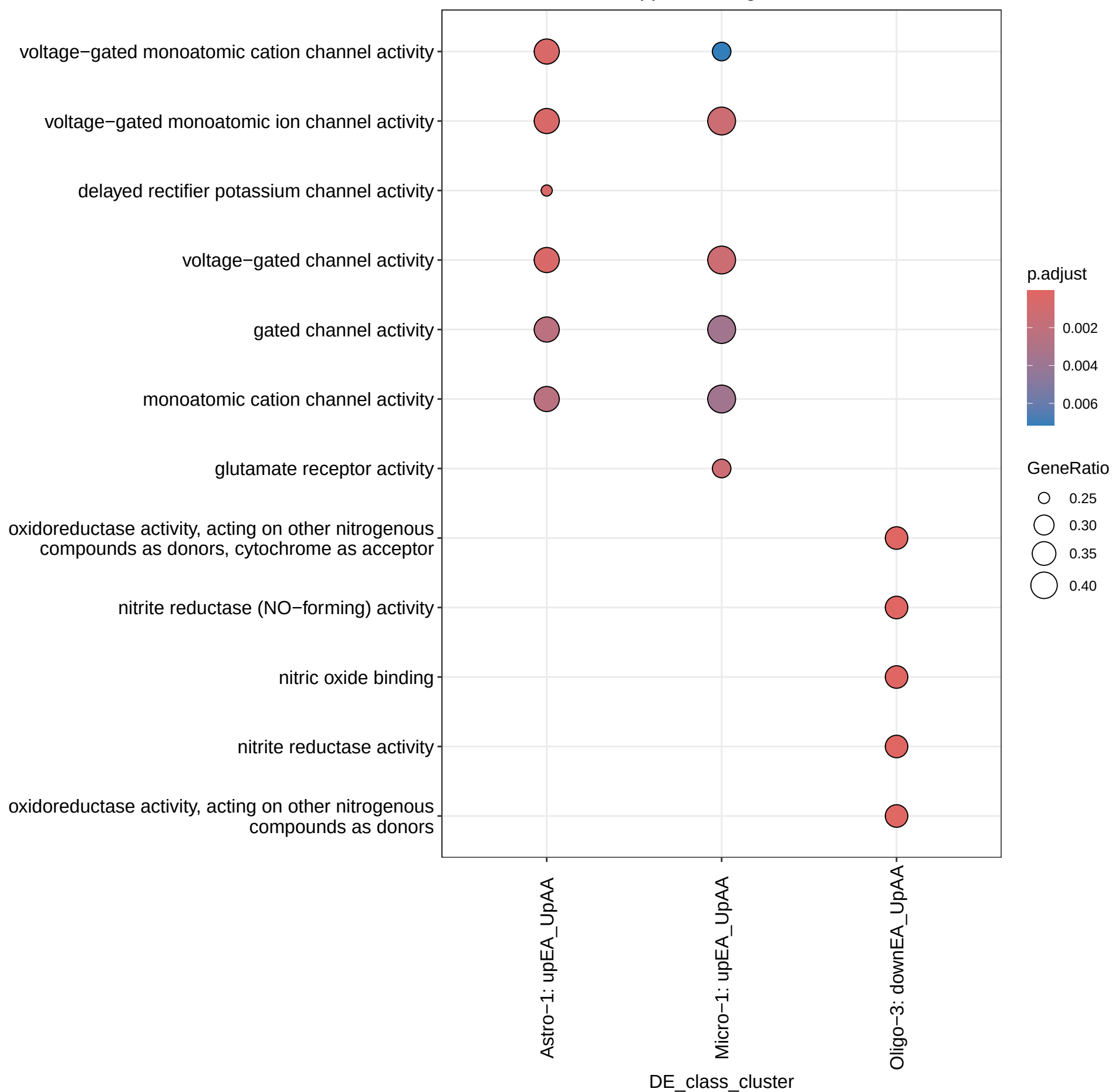
GO Enrichment: MF opposite, 2+ genes
