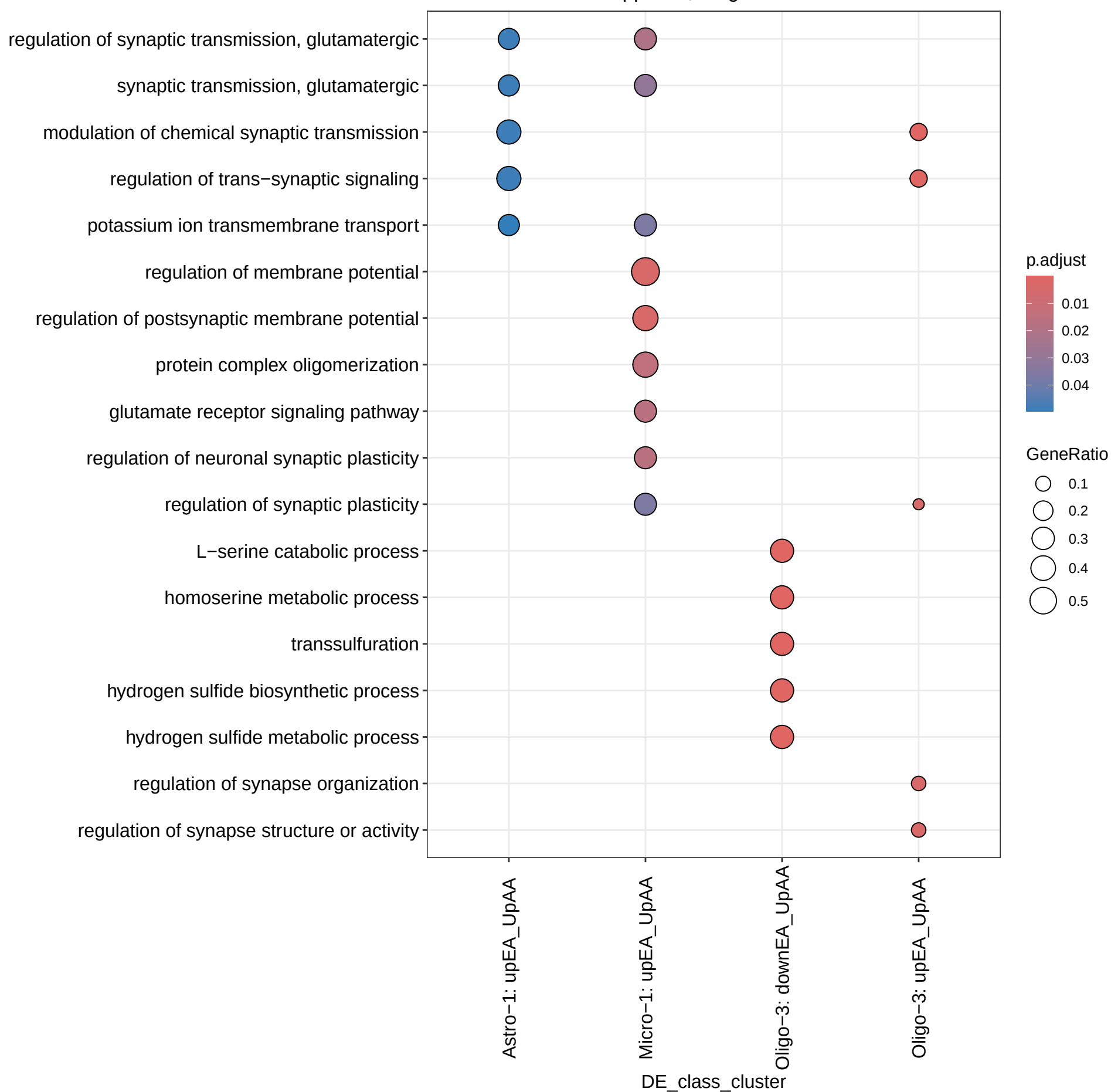
GO Enrichment: BP opposite, 2+ genes
