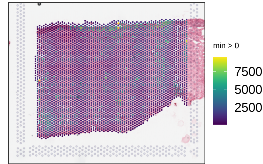
Br6263 sum_umi
