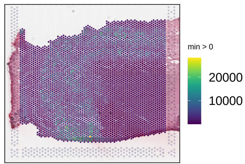
Br1039 sum_umi
