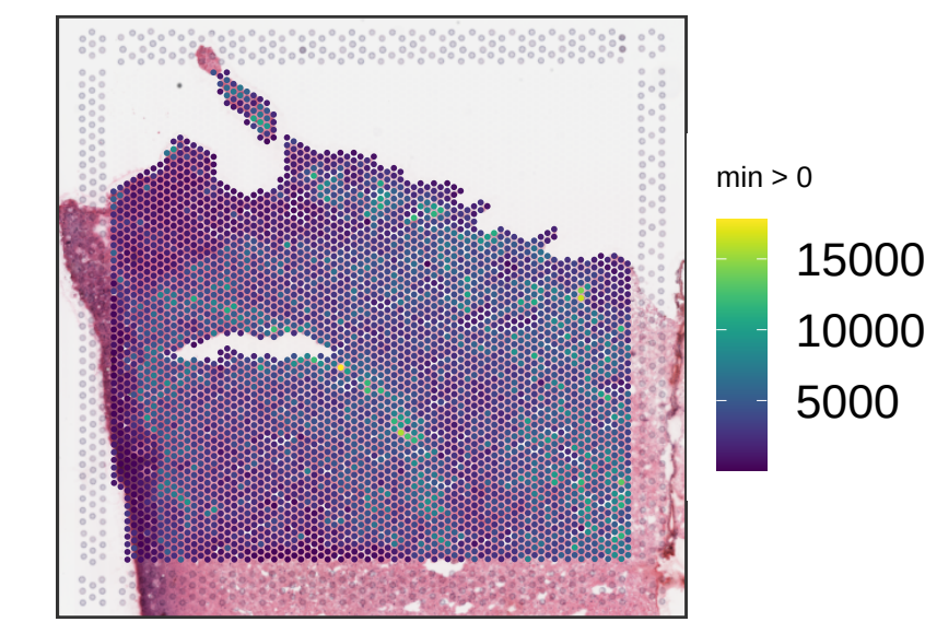
Br1706 sum_umi
