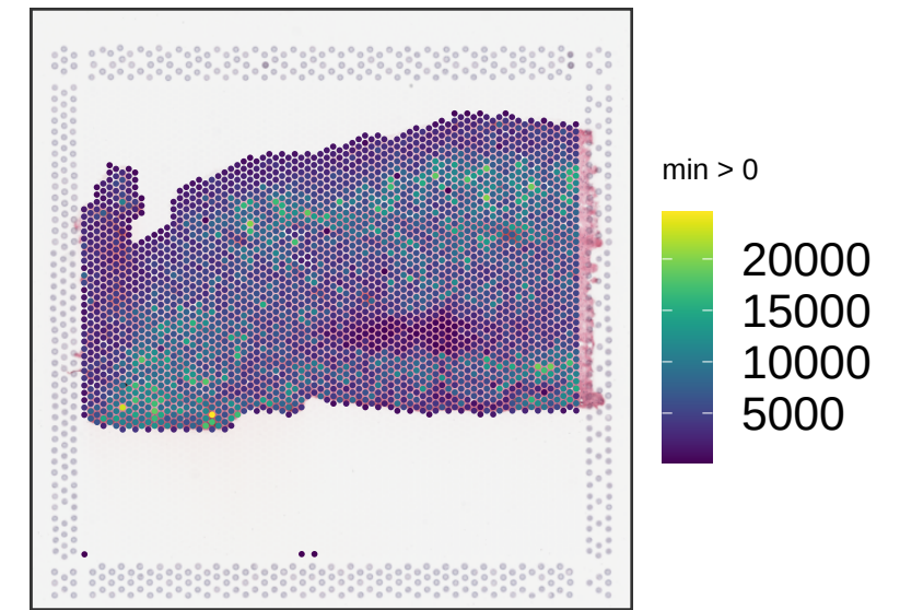
Br5367 sum_umi
