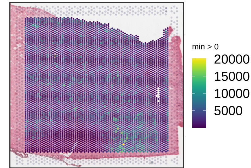
Br5212 sum_umi
