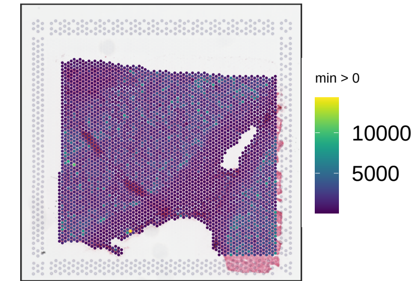
Br6321 sum_umi
