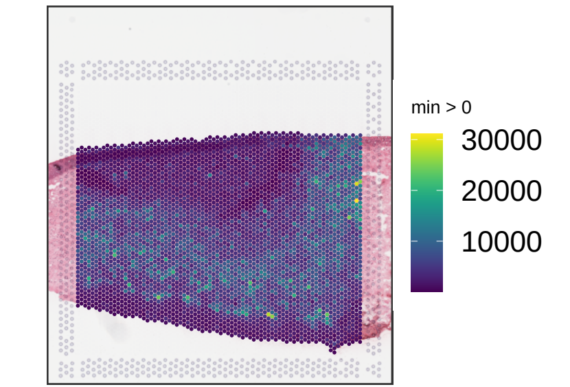
Br5854 sum_umi
