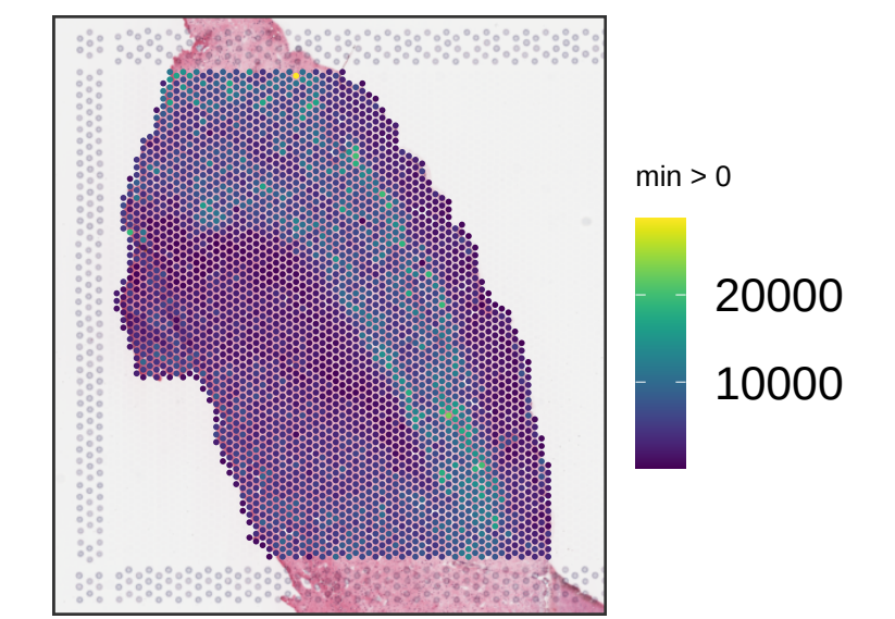
Br2305 sum_umi
