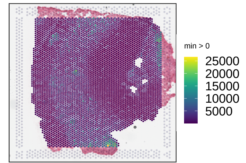
Br6538 sum_umi
