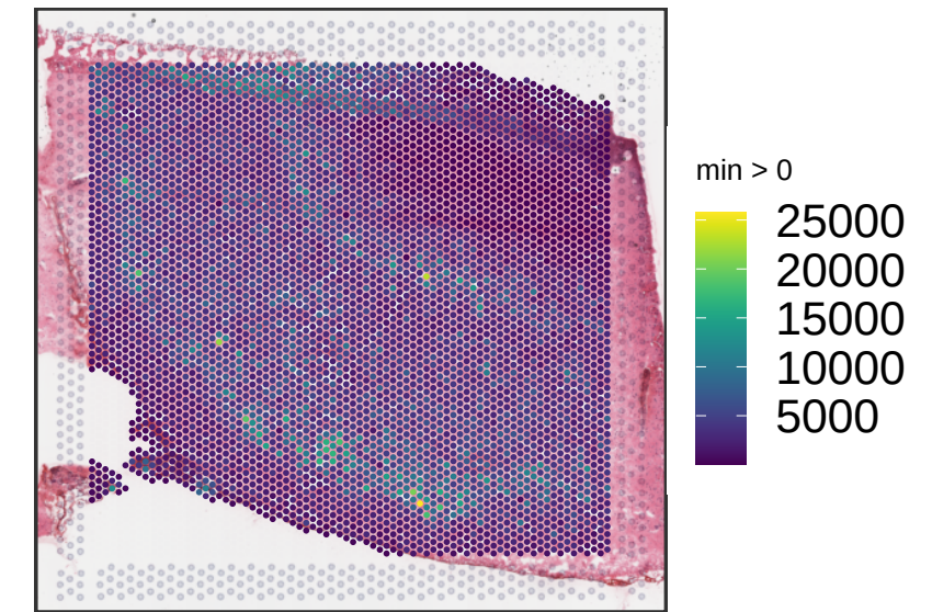
Br6098 sum_umi
