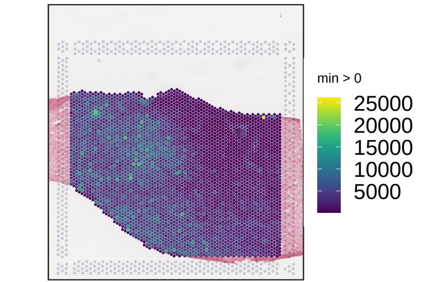
Br5832 sum_umi
