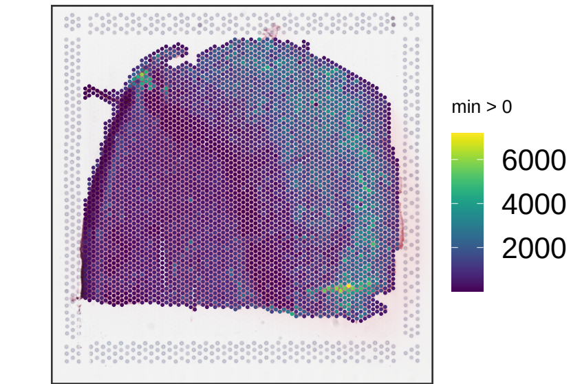
Br5276 sum_umi
