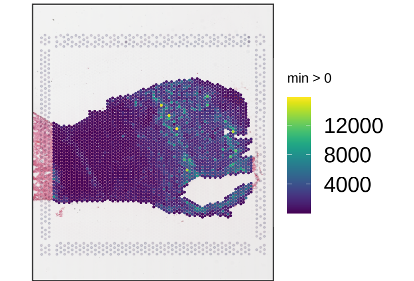
Br3974 sum_umi
