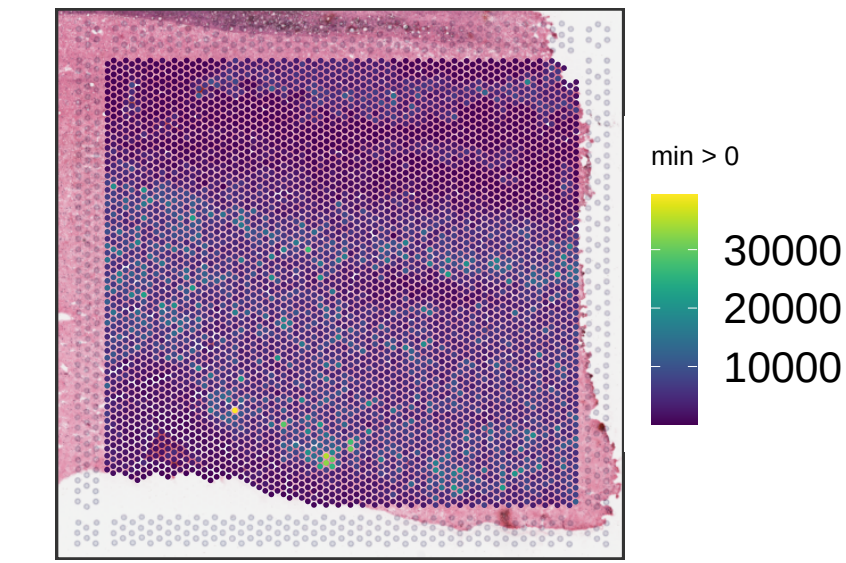
Br5941 sum_umi
