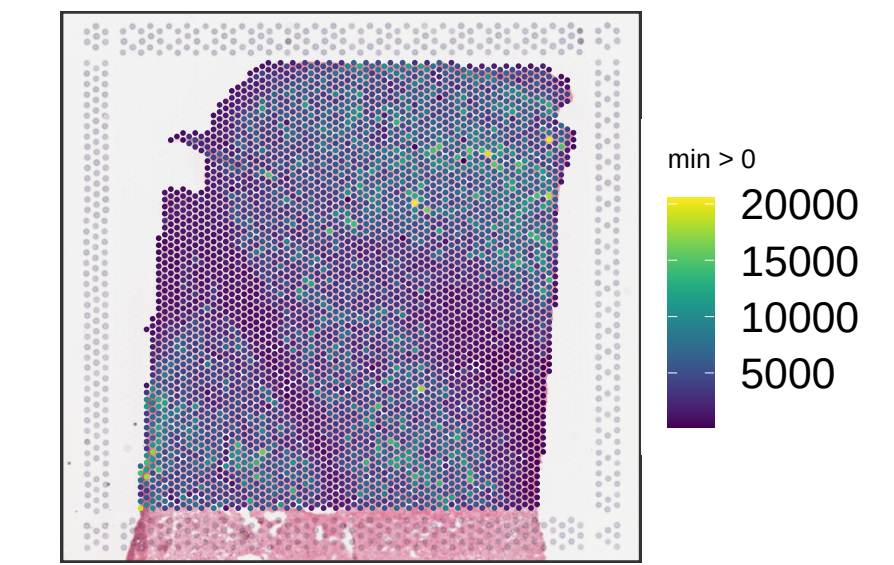
Br5460 sum_umi
