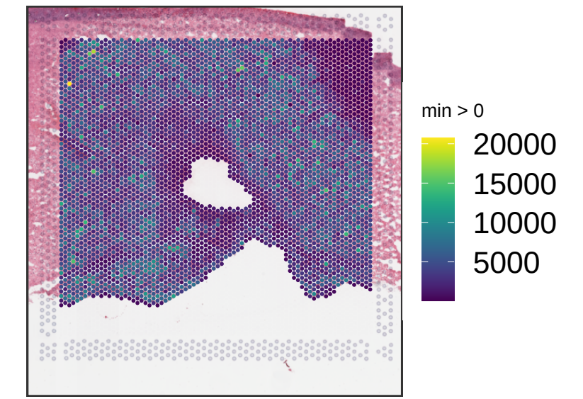
Br6085 sum_umi
