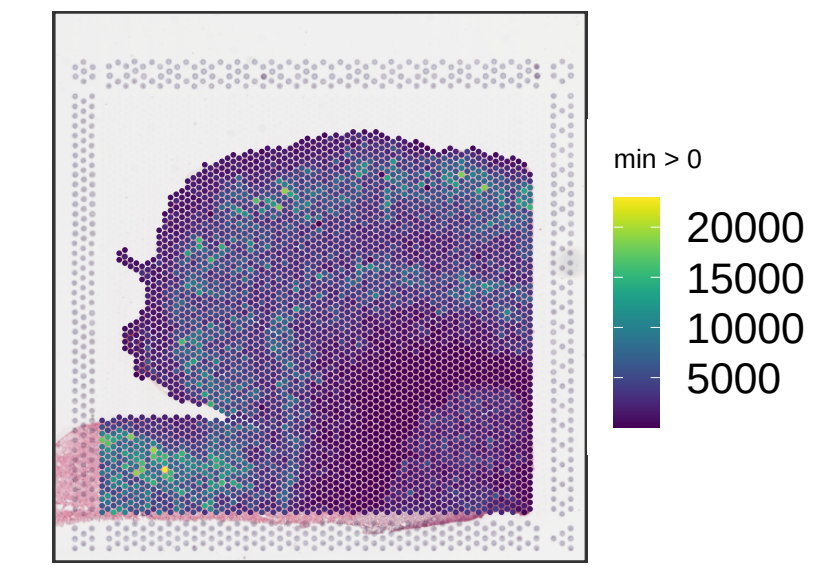
Br5517 sum_umi
