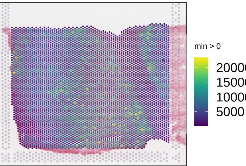
Br6476 sum_umi
