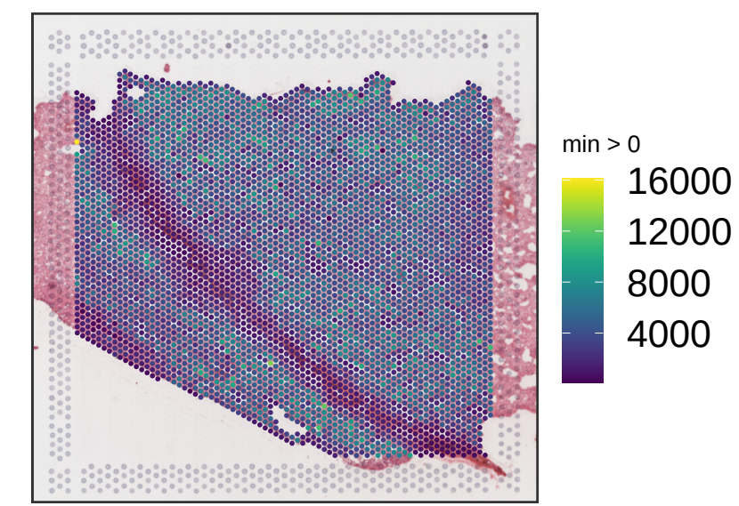
Br1691 sum_umi
