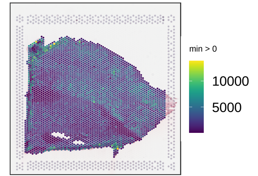
Br5712 sum_umi
