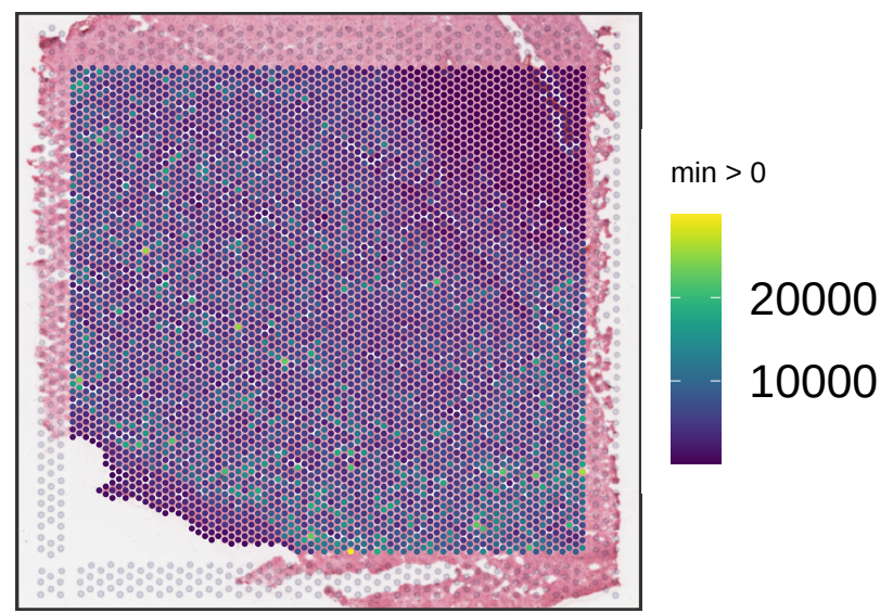
Br5599 sum_umi
