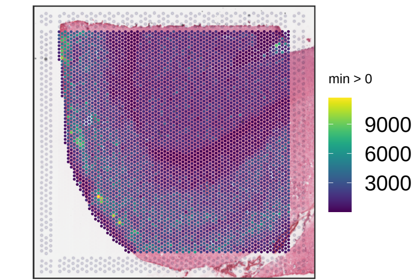
Br5529 sum_umi
