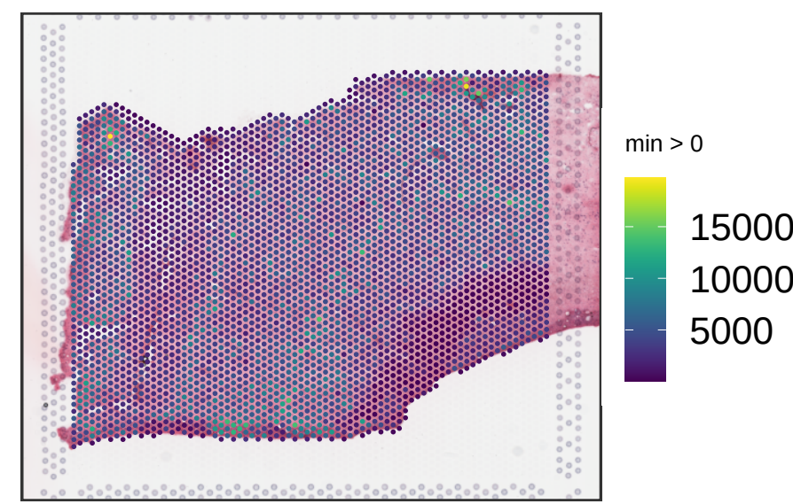
Br1556 sum_umi
