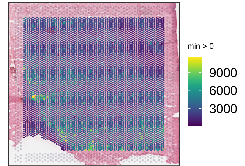
Br6161 sum_umi
