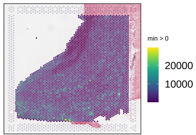
Br1289 sum_umi
