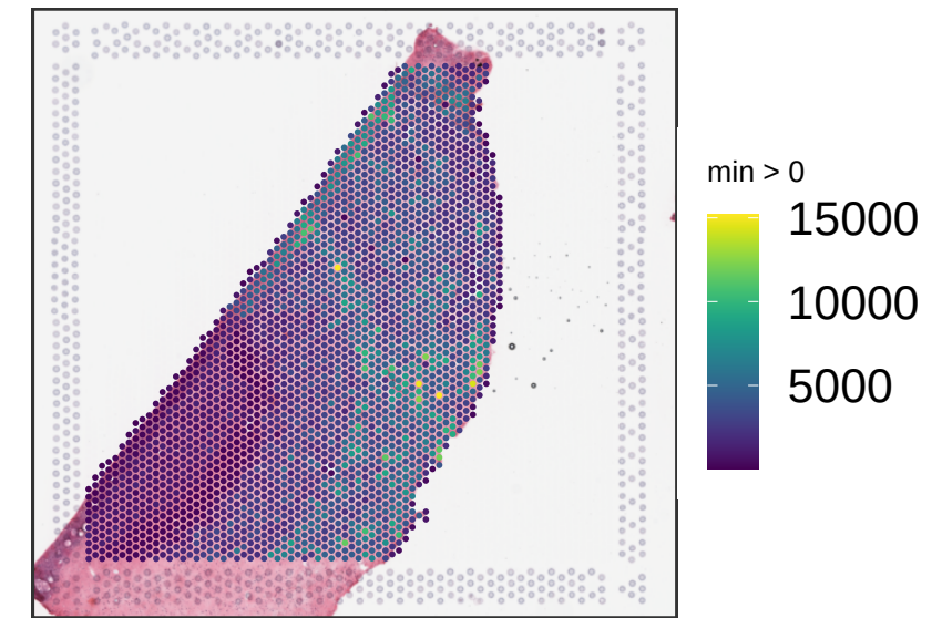
Br2582 sum_umi
