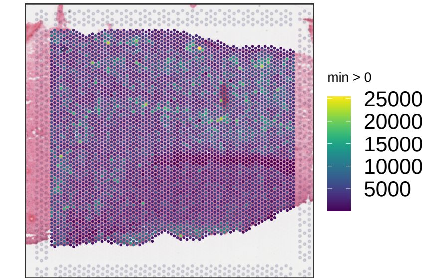
Br6423 sum_umi
