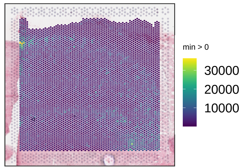
Br5426 sum_umi
