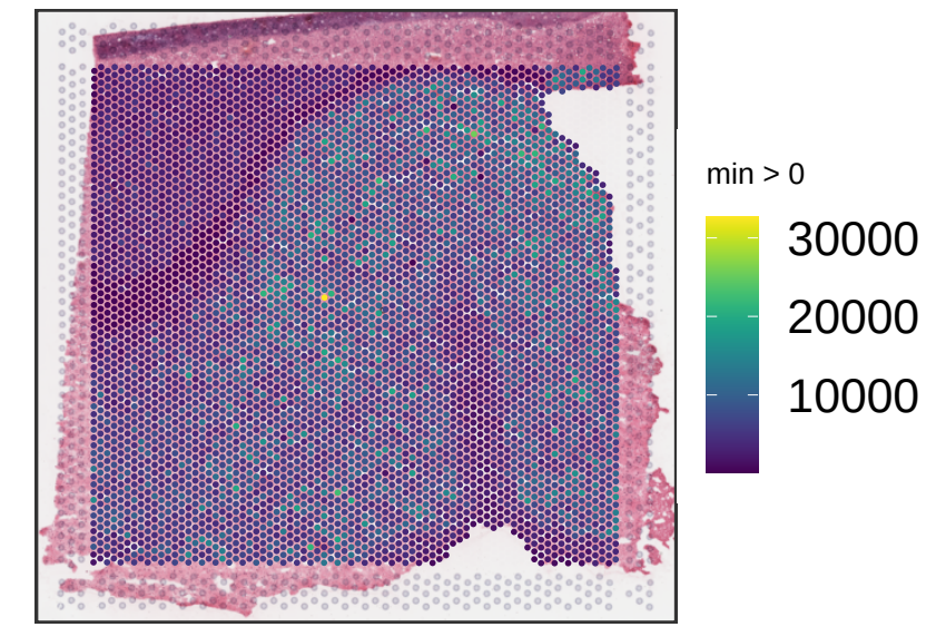
Br5634 sum_umi
