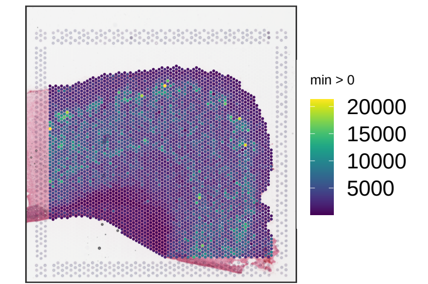
Br5415 sum_umi
