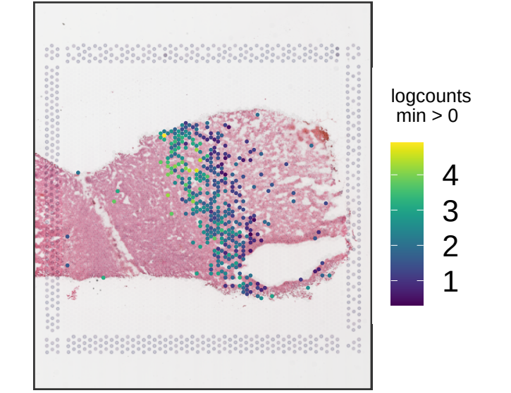
Br3974 KRT17
