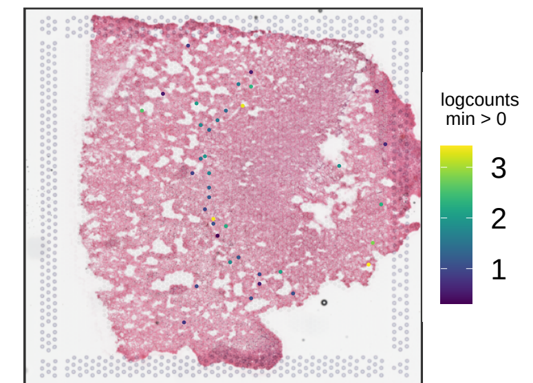
Br6538 KRT17
