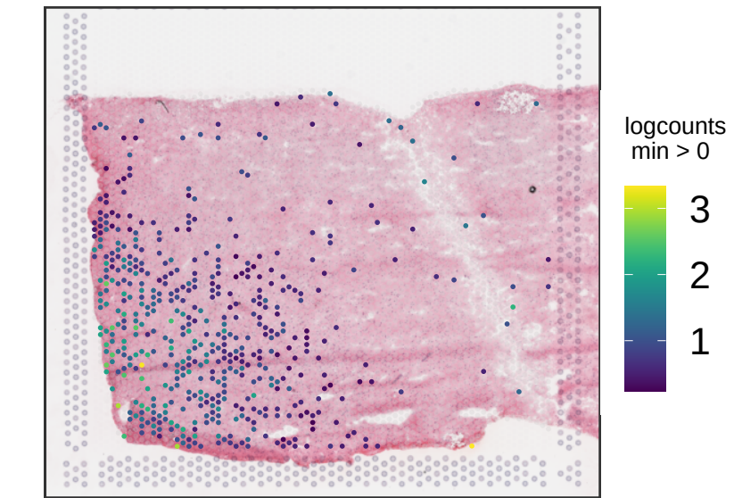
Br6476 KRT17
