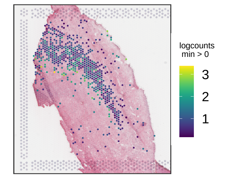
Br2305 KRT17
