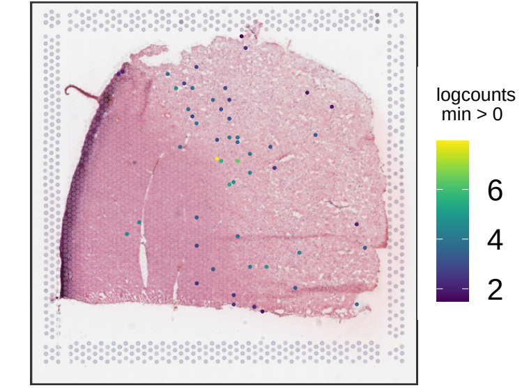
Br5276 KRT17
