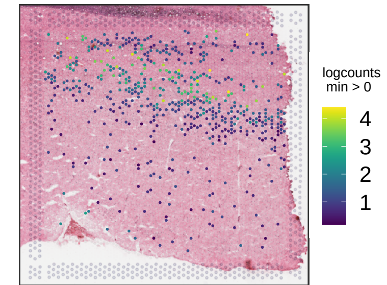
Br5941 KRT17
