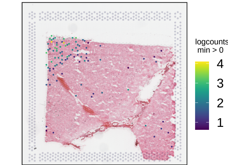
Br6321 KRT17
