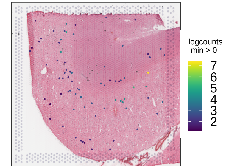
Br5529 KRT17
