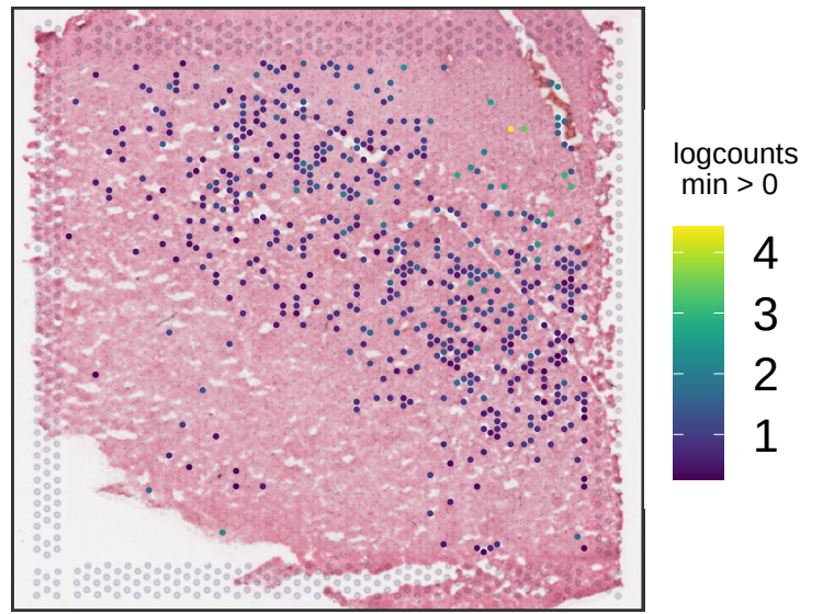
Br5599 KRT17
