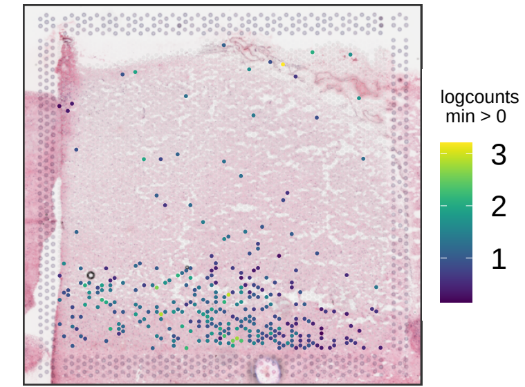
Br5426 KRT17
