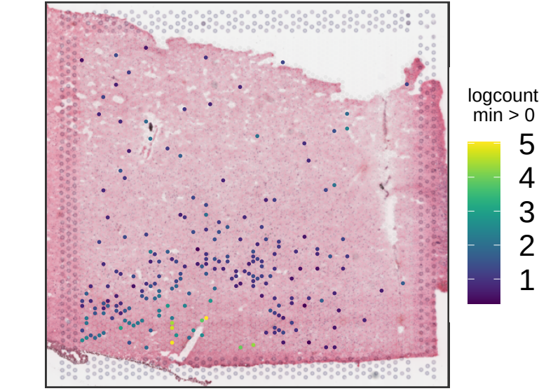
Br5212 KRT17
