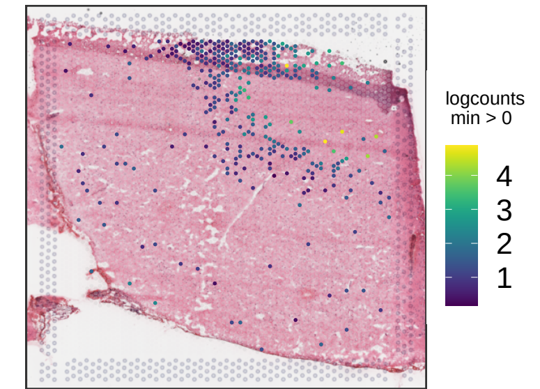
Br6098 KRT17
