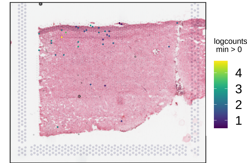
Br6263 KRT17
