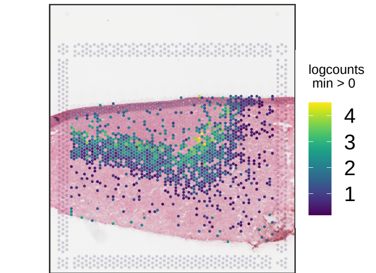
Br5854 KRT17
