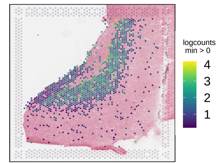
Br1289 KRT17
