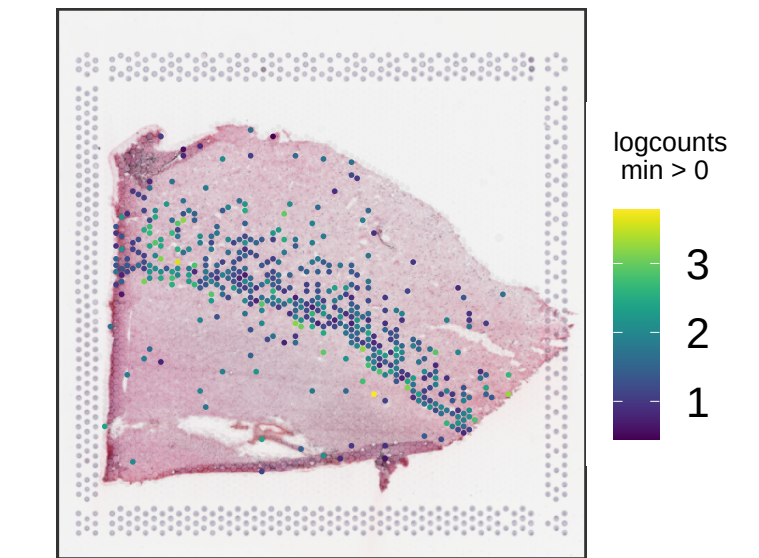
Br5712 KRT17
