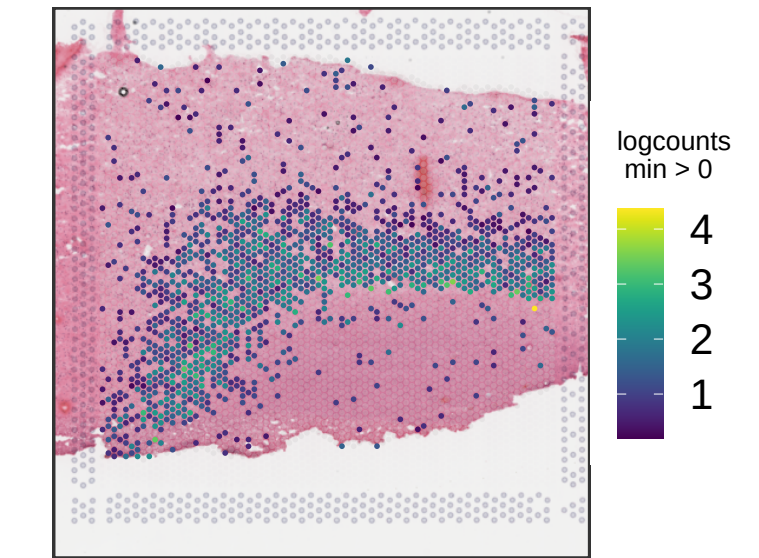
Br6423 KRT17
