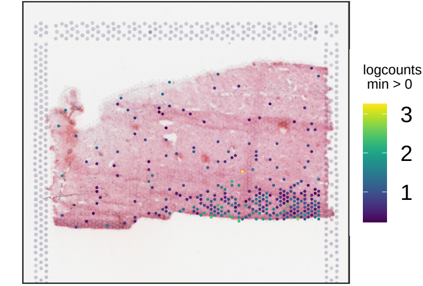
Br5367 KRT17
