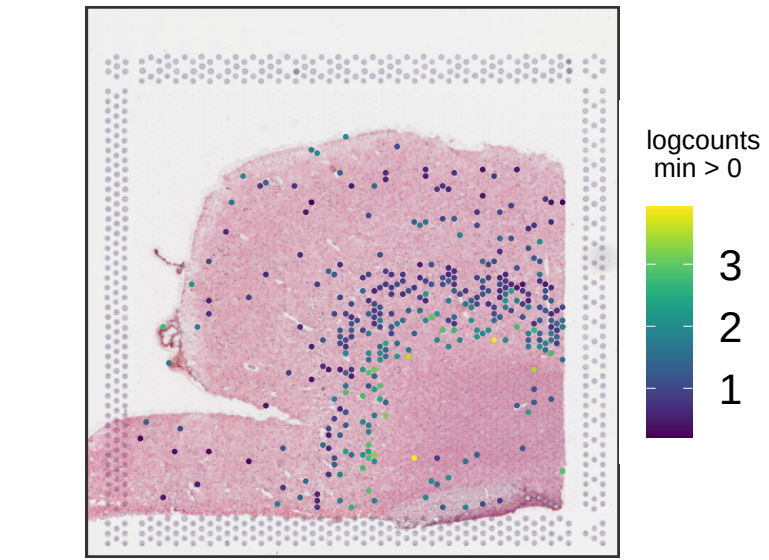
Br5517 KRT17
