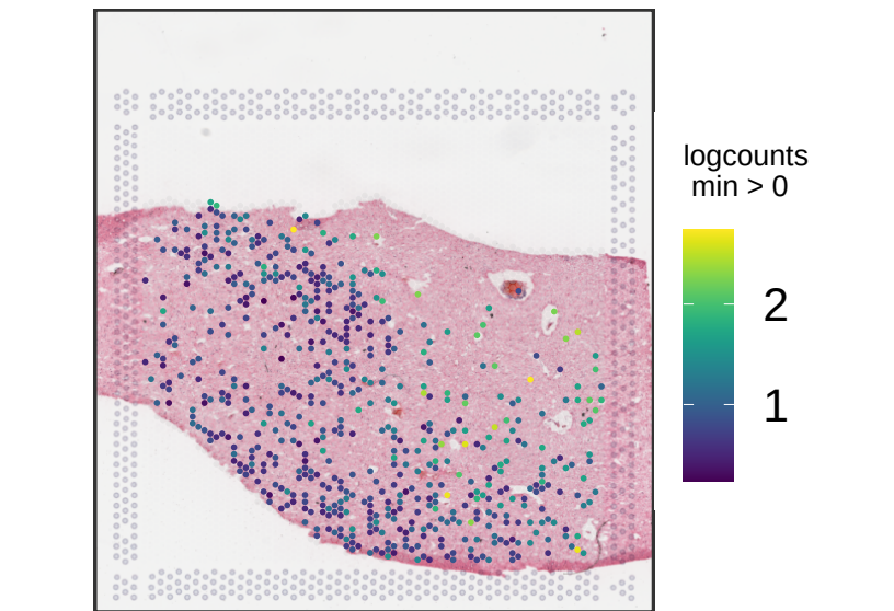
Br5832 KRT17
