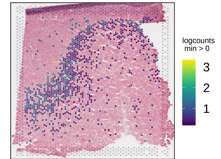
Br5634 KRT17
