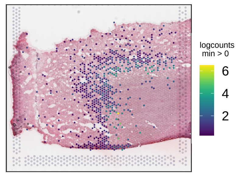
Br1039 KRT17
