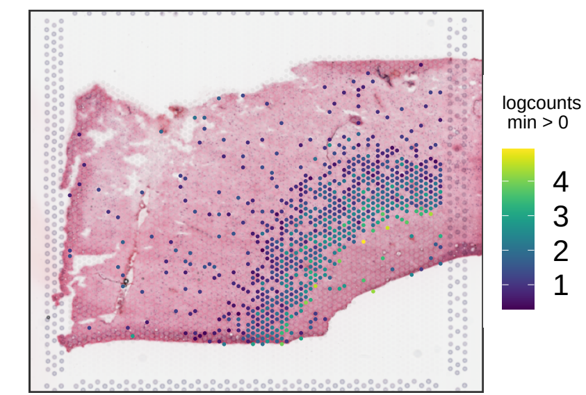
Br1556 KRT17
