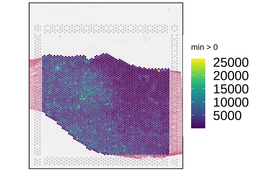
Br5832 sum_umi
