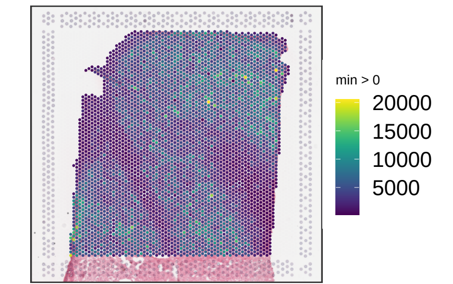
Br5460 sum_umi
