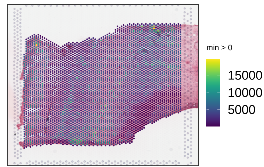
Br1556 sum_umi
