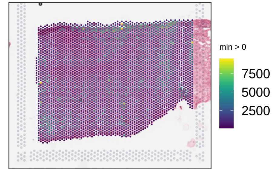
Br6263 sum_umi
