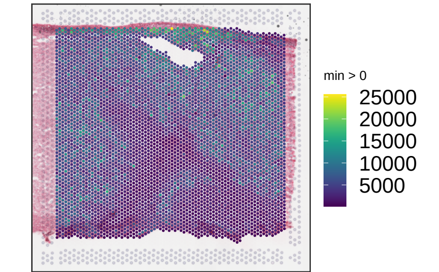
Br5161 sum_umi
