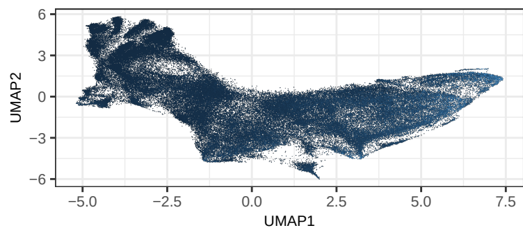
UMAP by expr_chrM_ratio
