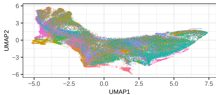
UMAP by sum_gene
