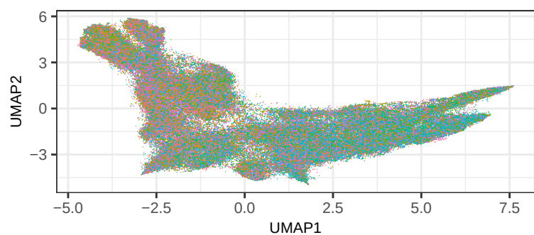
HARMONY-UMAP by capture_id
