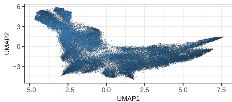
HARMONY-UMAP by sum_umi
