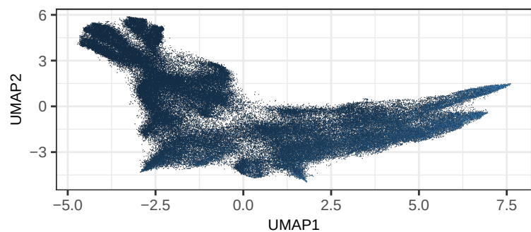
HARMONY-UMAP by expr_chrM_ratio
