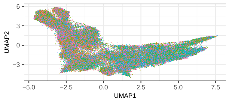
HARMONY-UMAP by sum_gene
