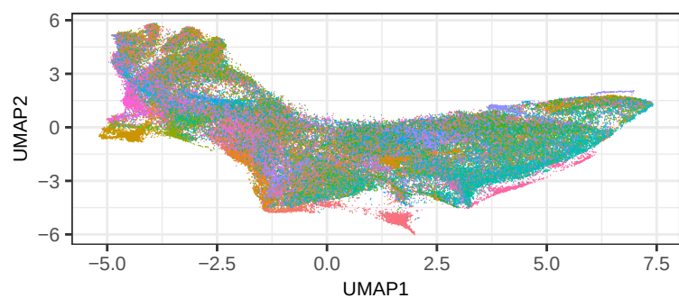
UMAP by capture_id
