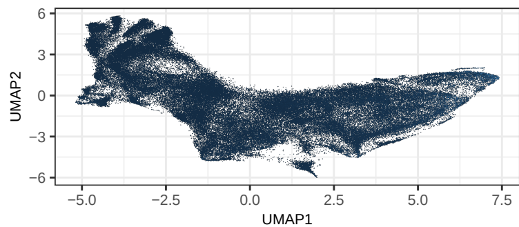
UMAP by sum_umi
