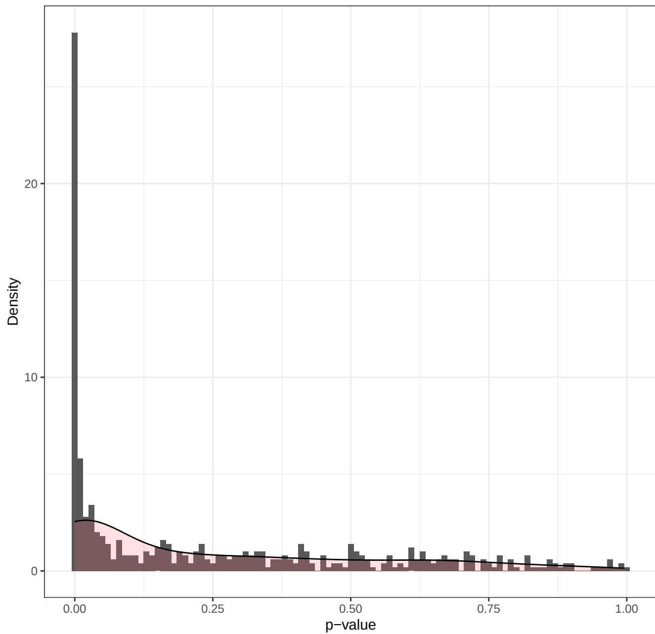
p-value distribution
