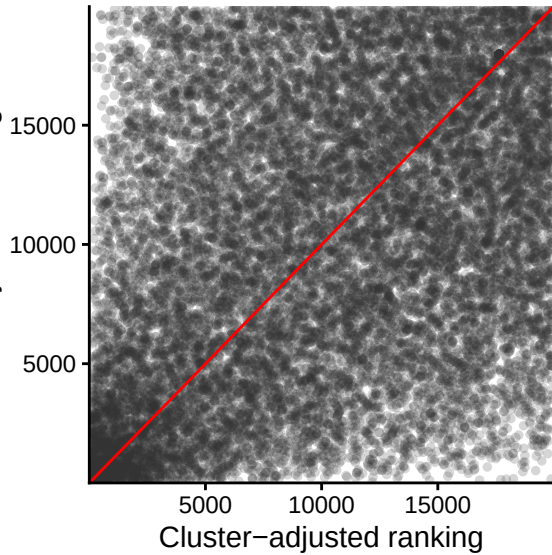
SV-adjusted ranking
