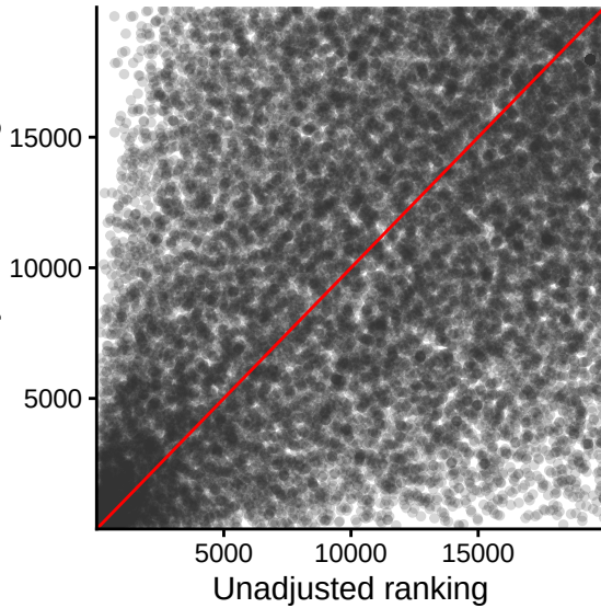
SV-adjusted ranking
