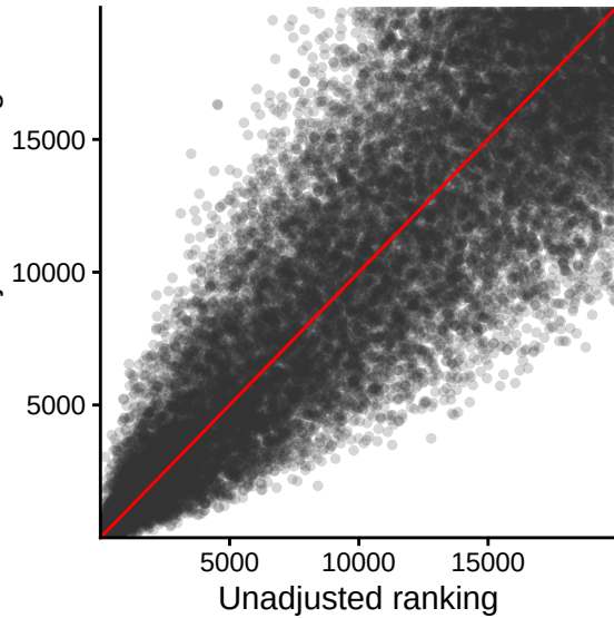
Cluster-adjusted ranking
