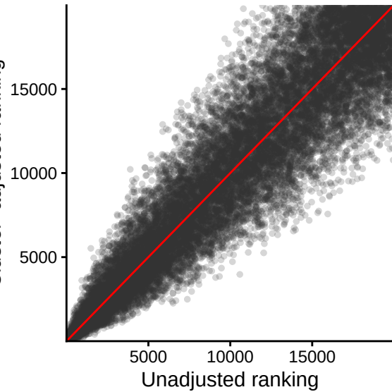
SV-adjusted ranking
