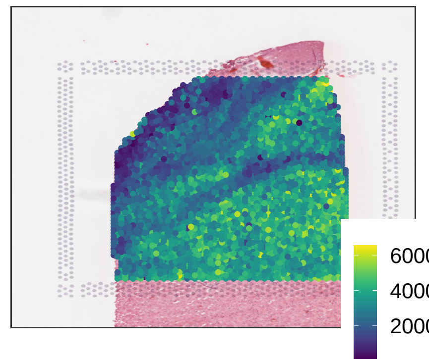
V13M06-388_B1 sum_gene
