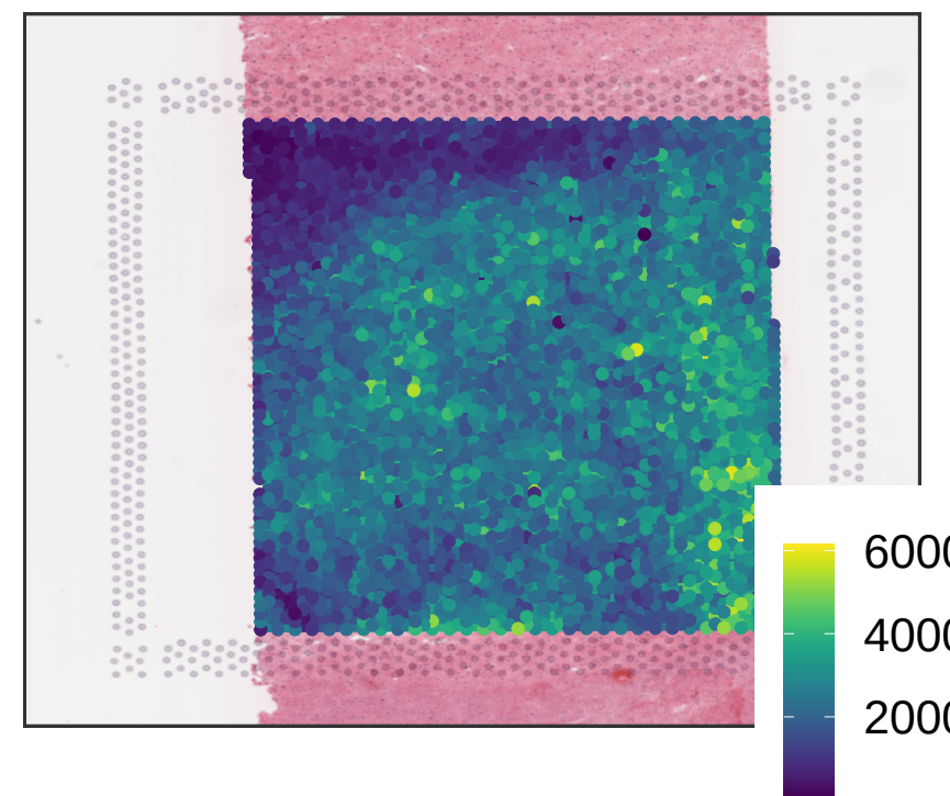
V13M06-387_B1 sum_gene
