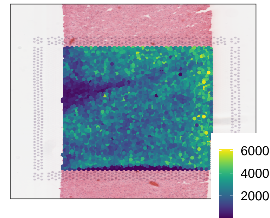
V13M06-388_D1 sum_gene
