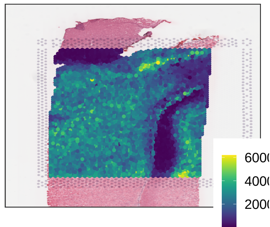
V13M06-388_A1 sum_gene
