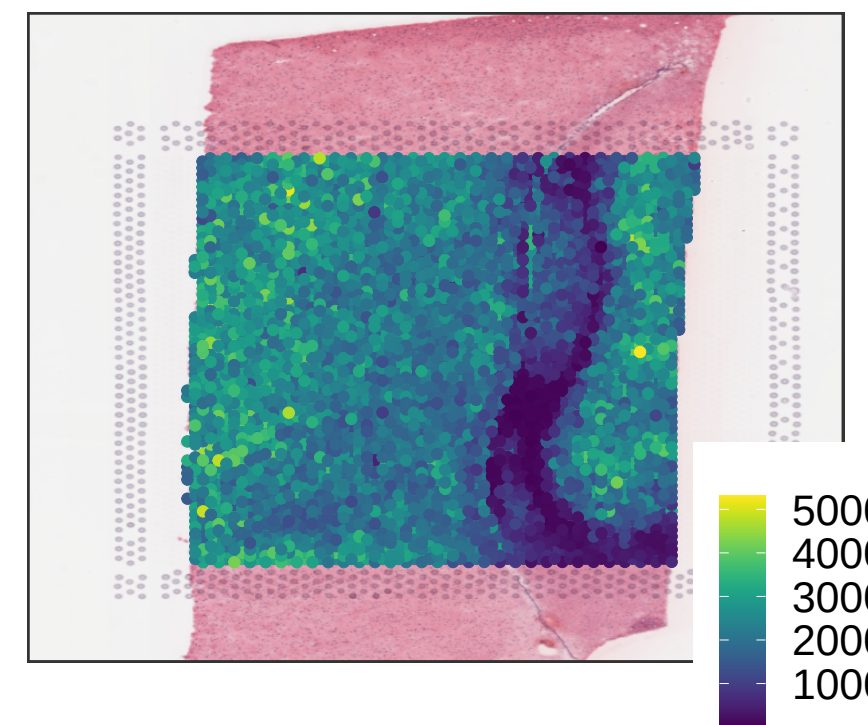
V13M06-388_C1 sum_gene
