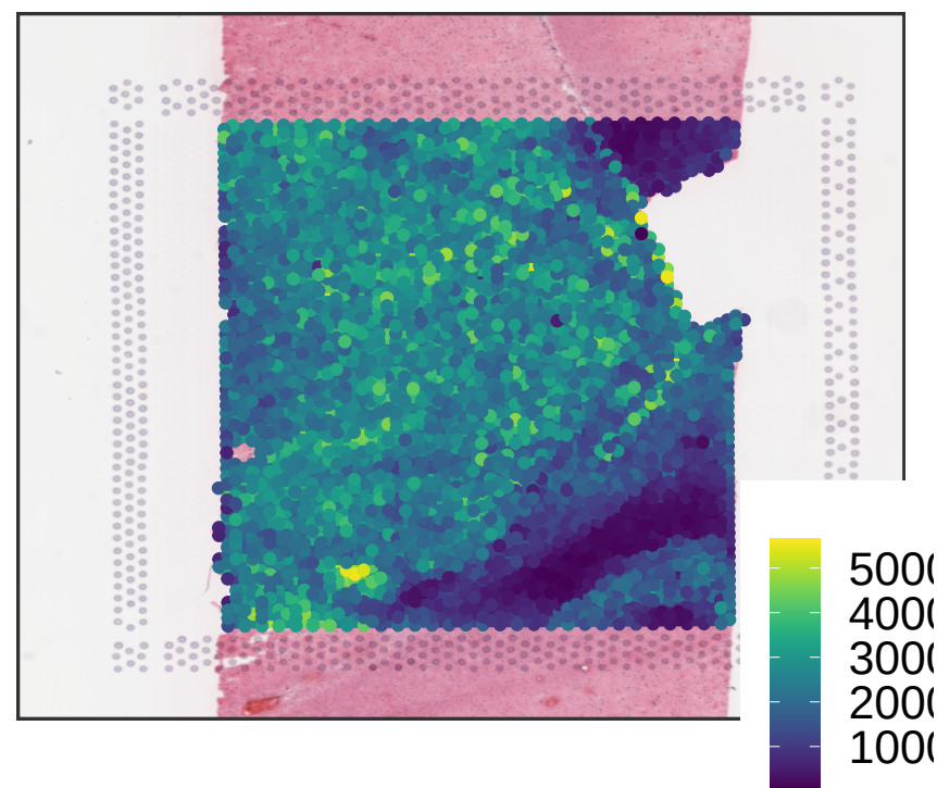
V13M06-387_A1 sum_gene
