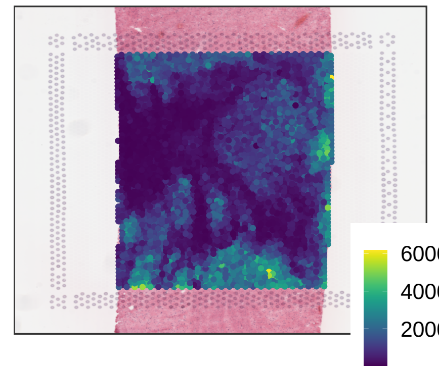
V13M06-387_C1 sum_gene
