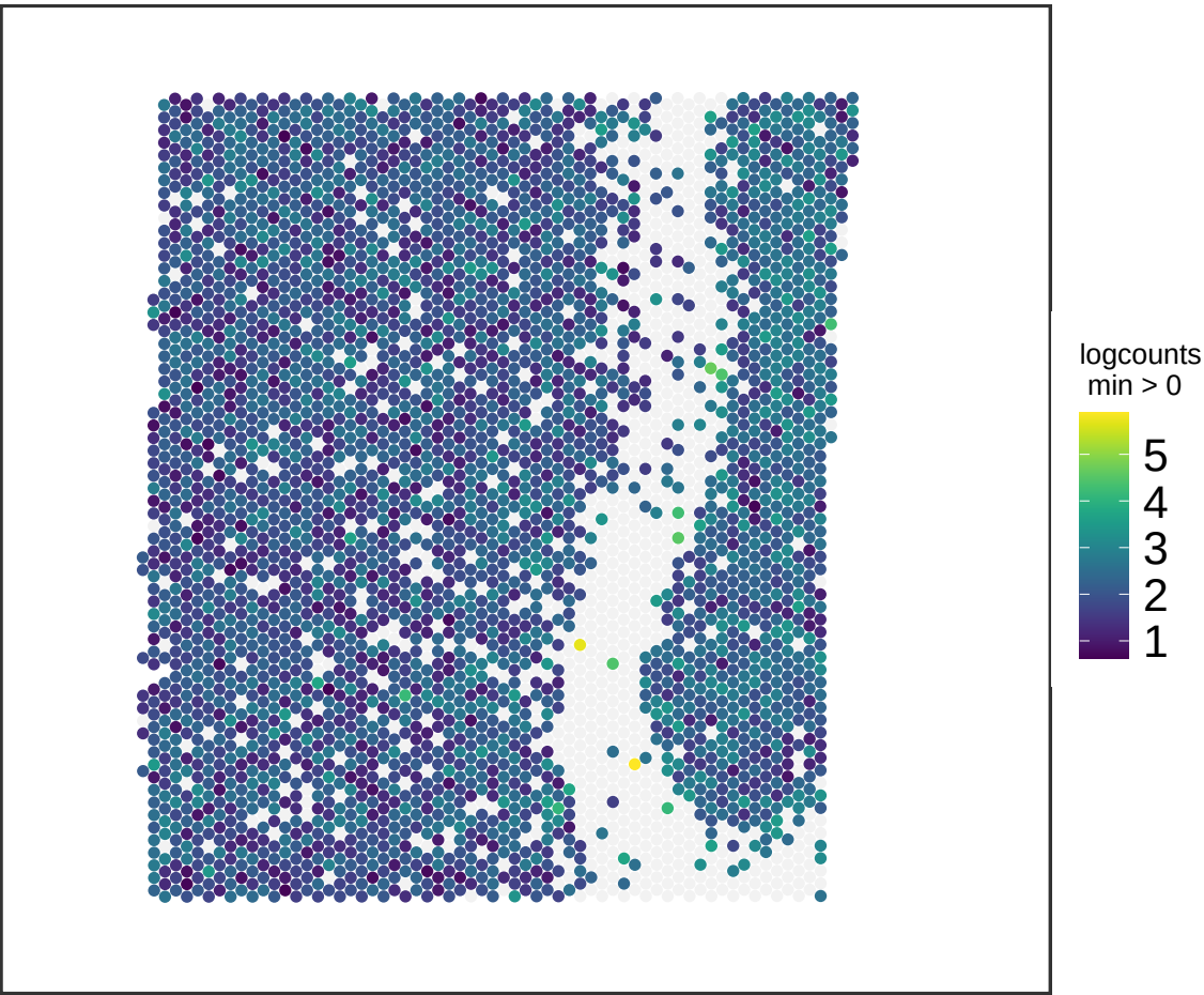
V13M06-388_C1 BASP1
