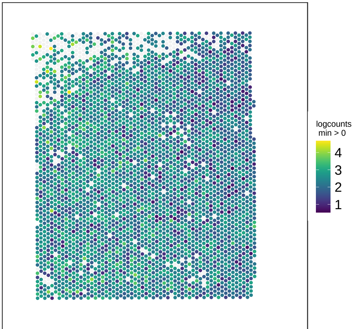
V13M06-387_B1 BASP1
