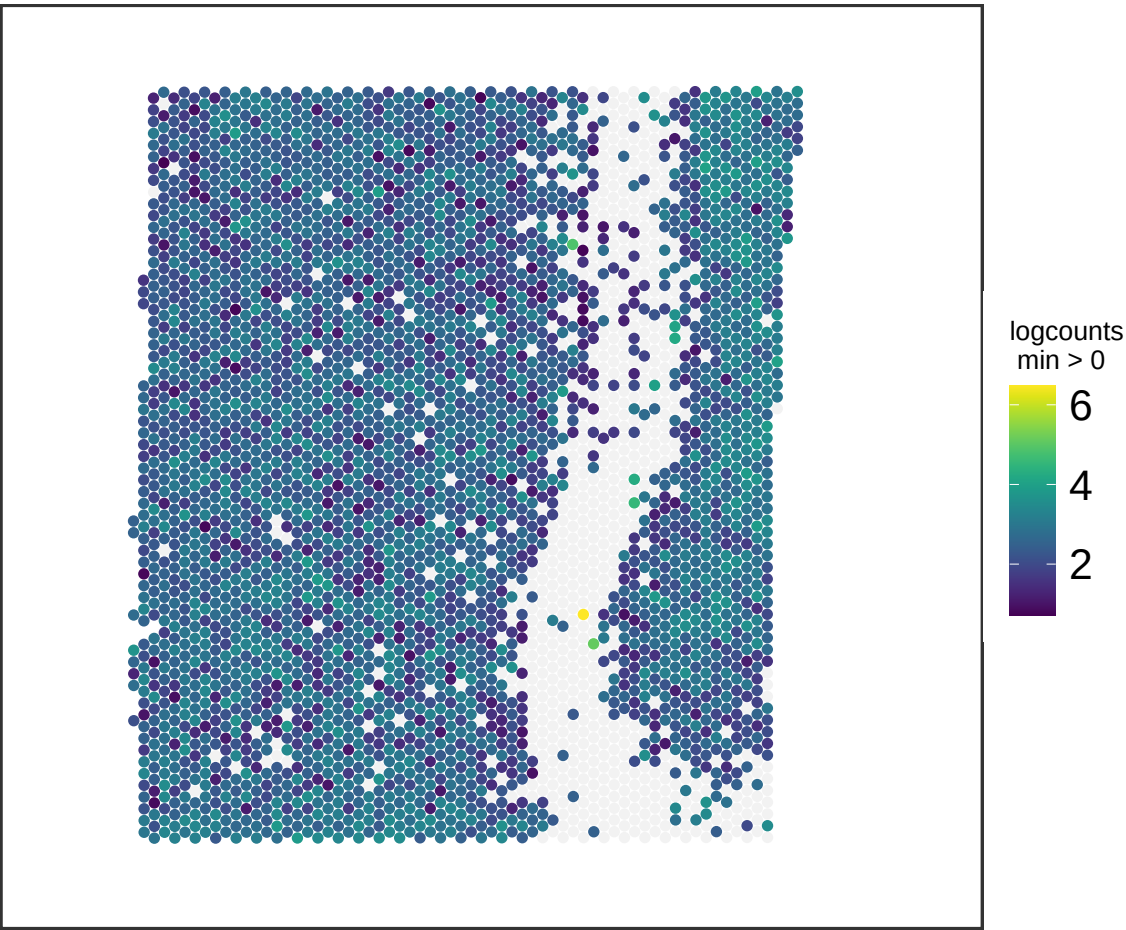
V13M06-388_C1 SLC17A7
