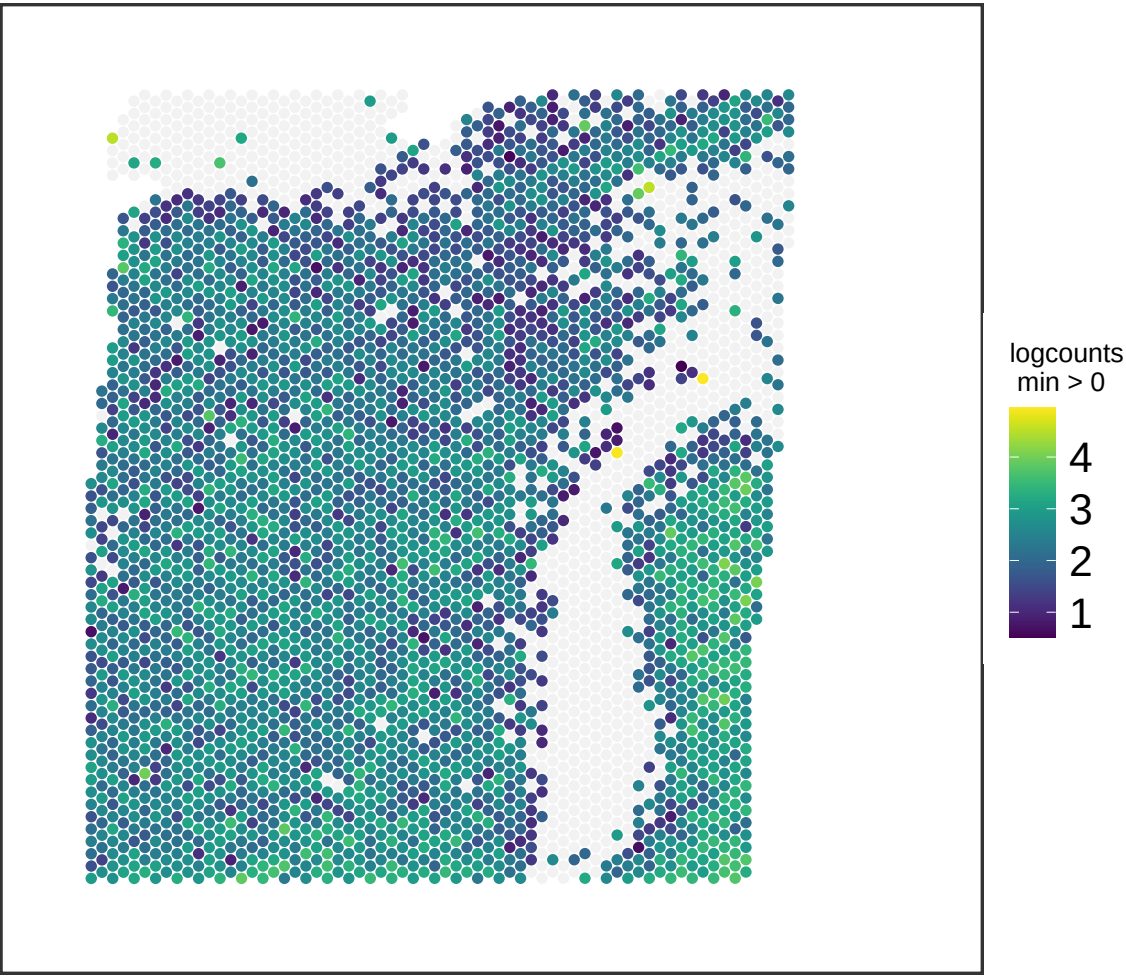
V13M06-388_A1 SLC17A7
