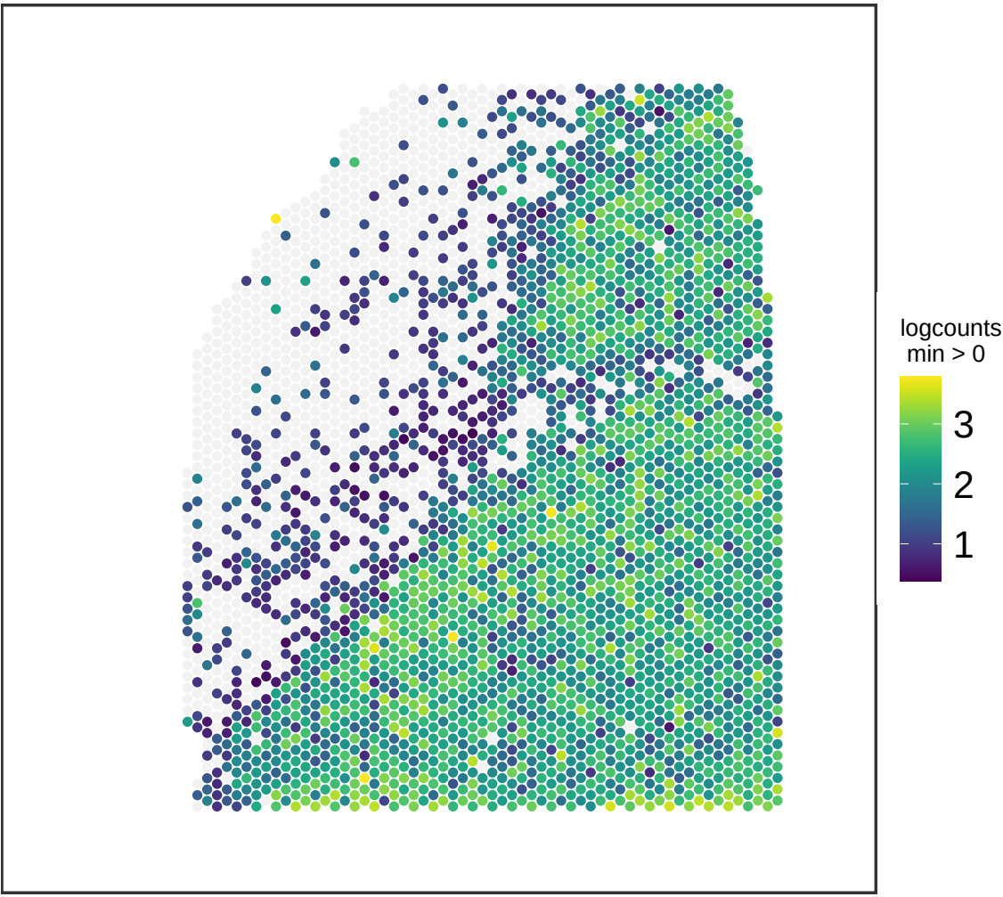
V13M06-388_B1 SLC17A7
