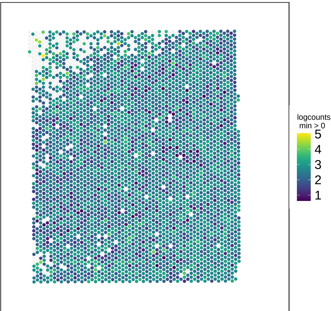
V13M06-387_B1 SLC17A7
