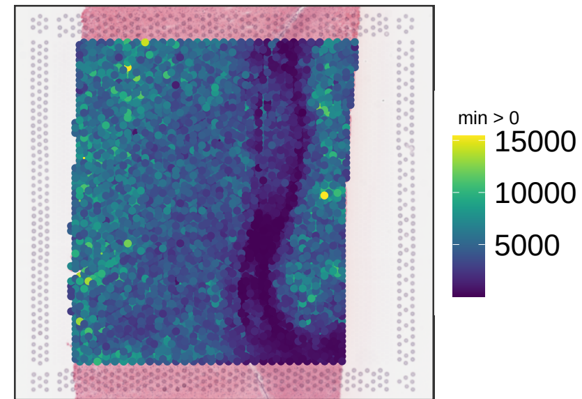
V13M06-388_C1 sum_umi
