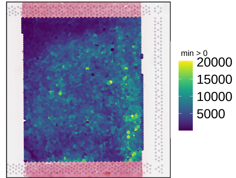
V13M06-387_B1 sum_umi
