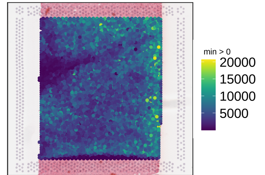
V13M06-388_D1 sum_umi
