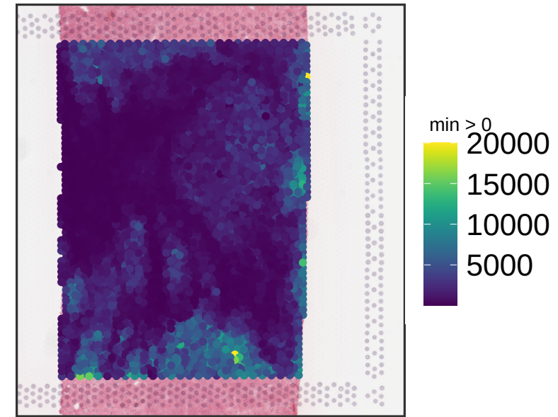
V13M06-387_C1 sum_umi
