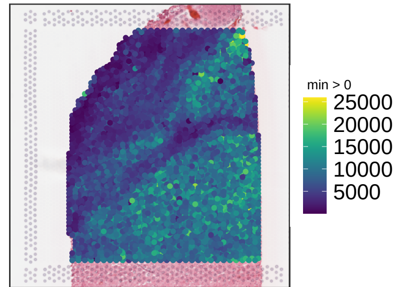
V13M06-388_B1 sum_umi
