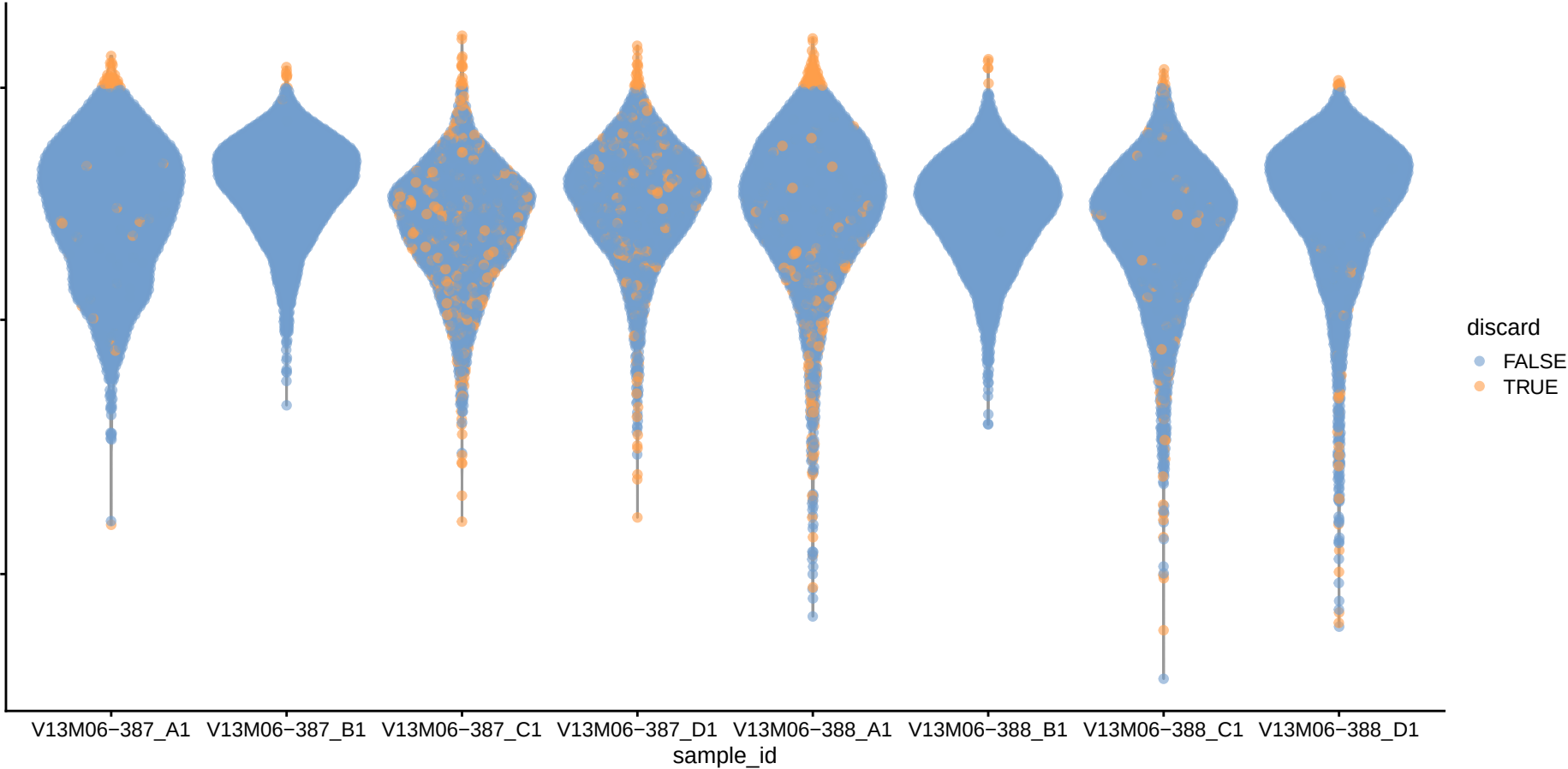
Mitochondrial Percent
