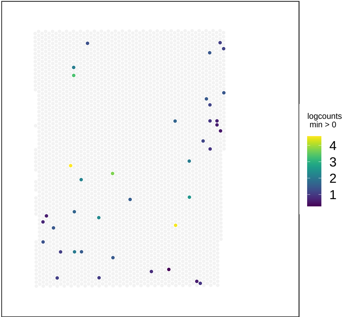
V13M06-387_C1 TMEM132D
