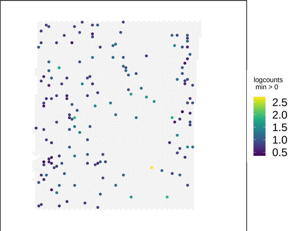
V13M06-388_C1 TMEM132D
