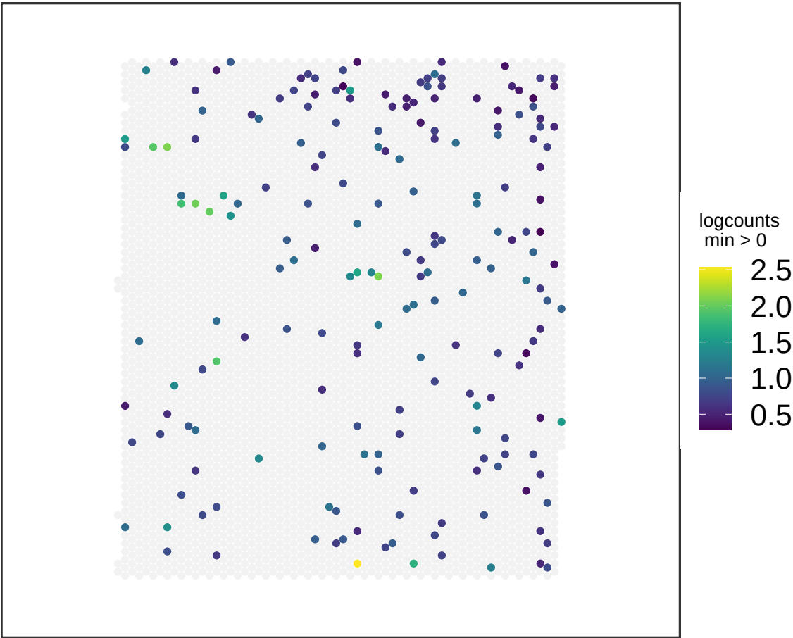
V13M06-388_D1 TMEM132D
