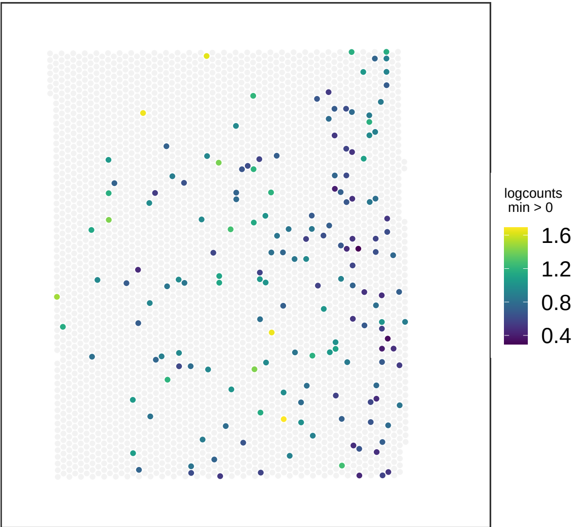
V13M06-387_B1 TMEM132D
