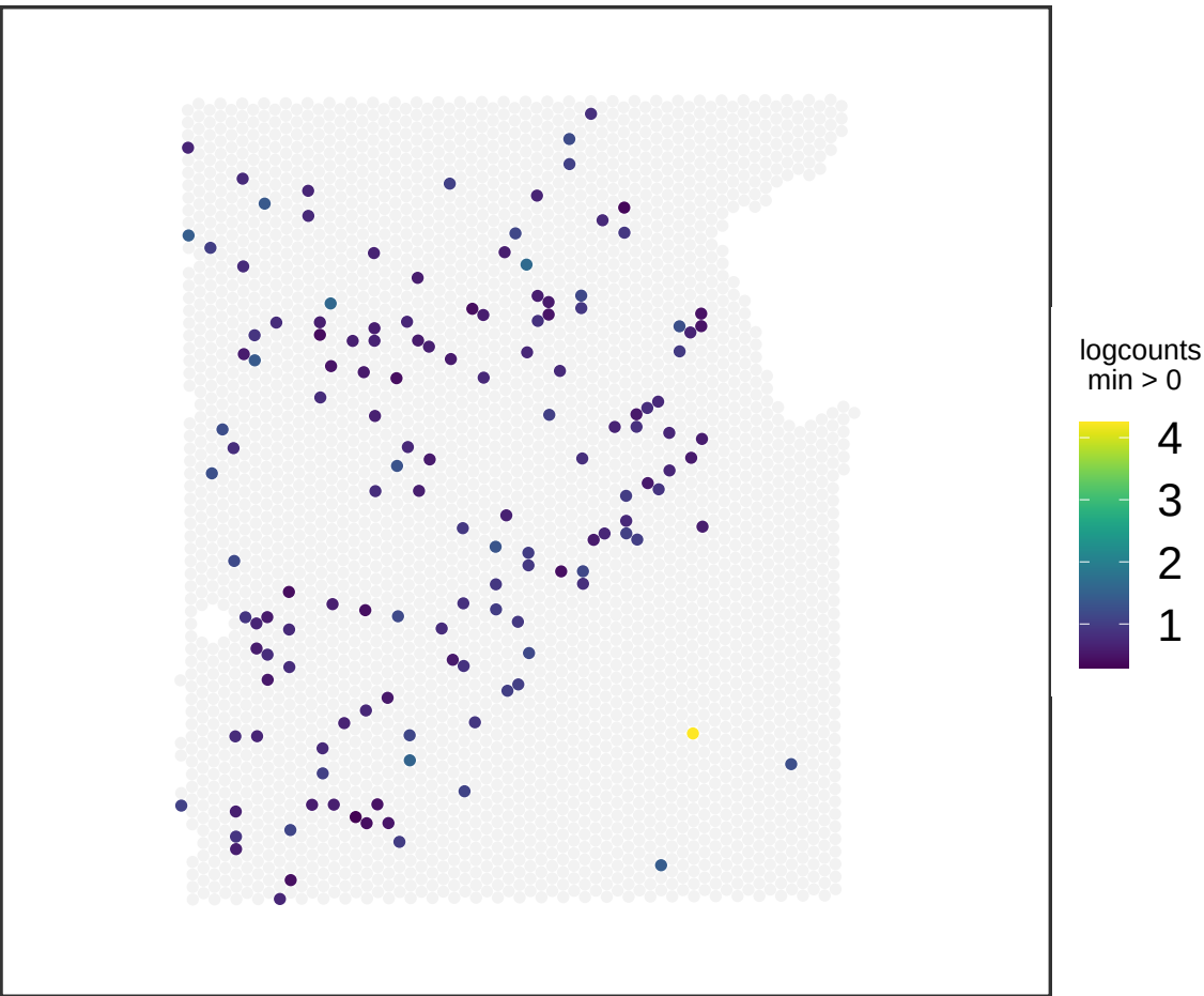
V13M06-387_A1 TMEM132D
