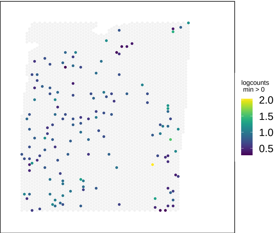
V13M06-388_A1 TMEM132D
