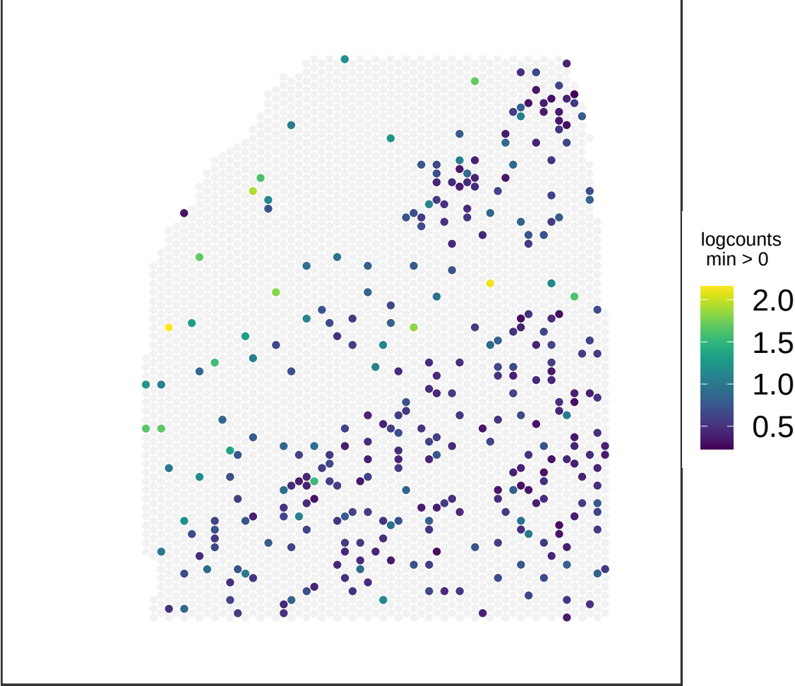
V13M06-388_B1 TMEM132D
