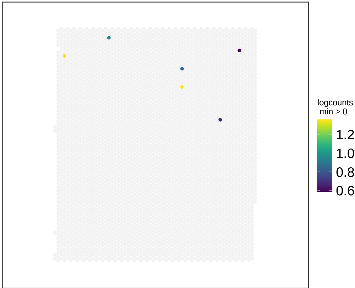
V13M06-388_D1 FAM183A
