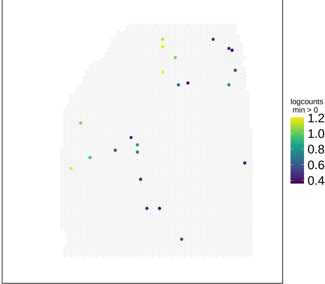
V13M06-388_B1 FAM183A
