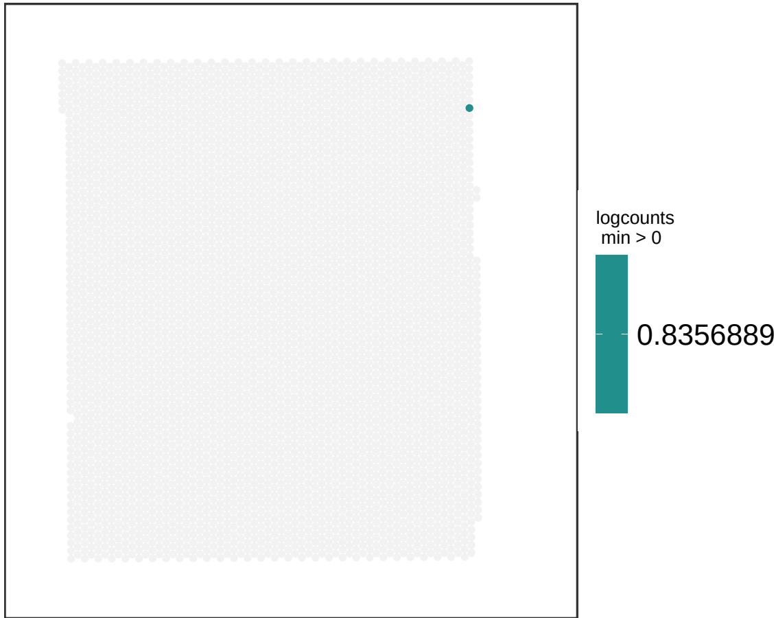
V13M06-387_B1 FAM183A
