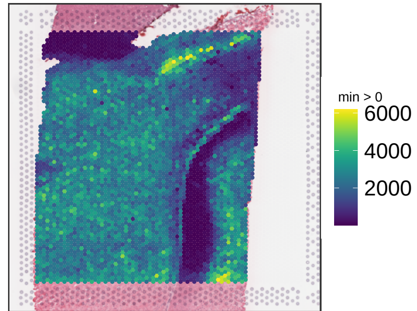
V13M06-388_A1 sum_gene
