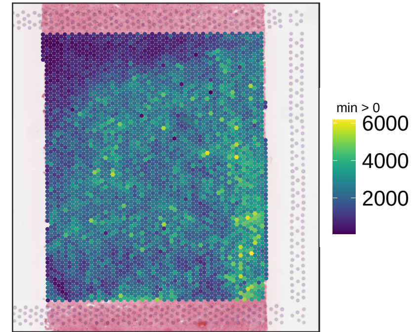
V13M06-387_B1 sum_gene
