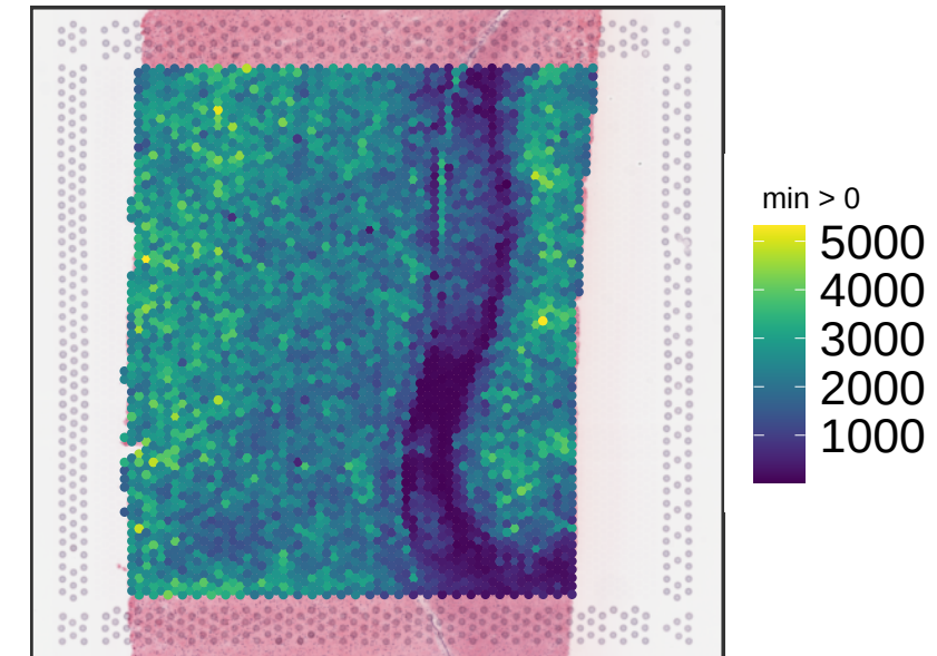
V13M06-388_C1 sum_gene
