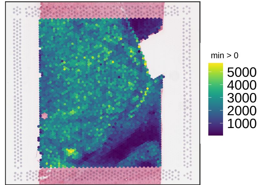
V13M06-387_A1 sum_gene
