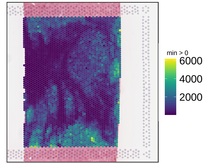
V13M06-387_C1 sum_gene
