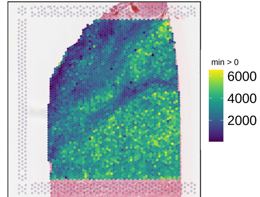
V13M06-388_B1 sum_gene
