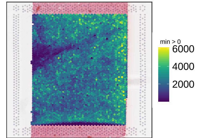
V13M06-388_D1 sum_gene
