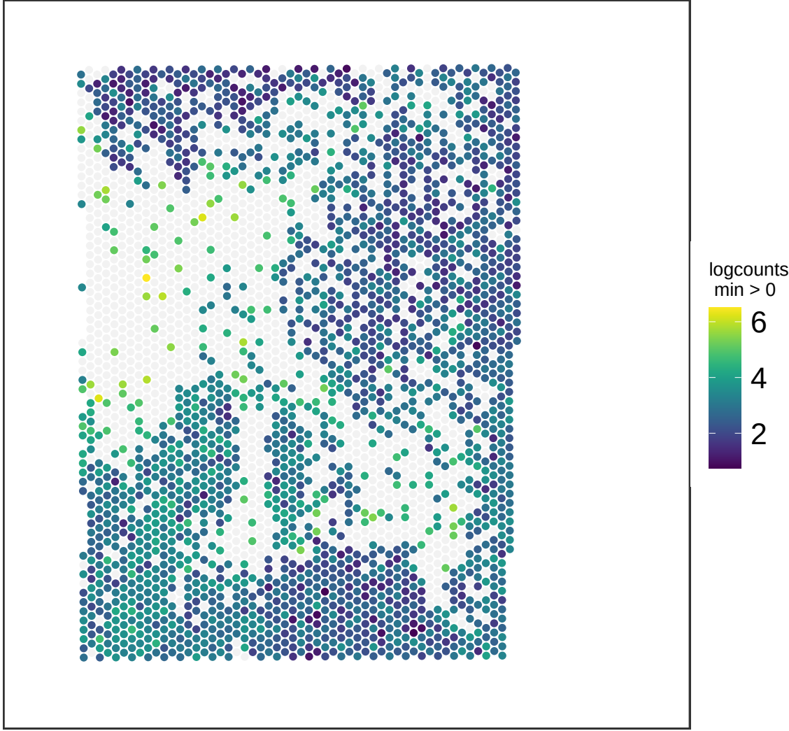
V13M06-387_C1 CAMK2N1
