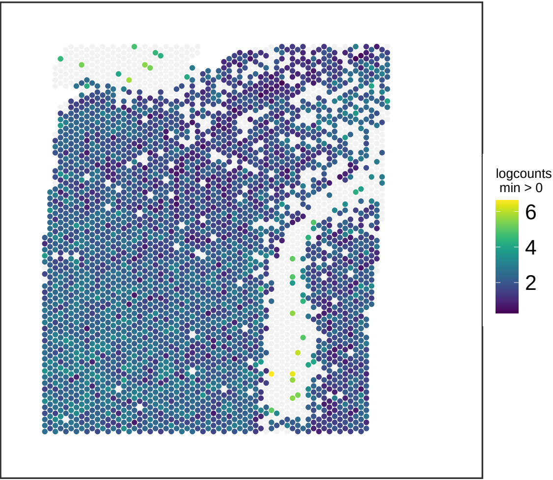
V13M06-388_A1 CAMK2N1
