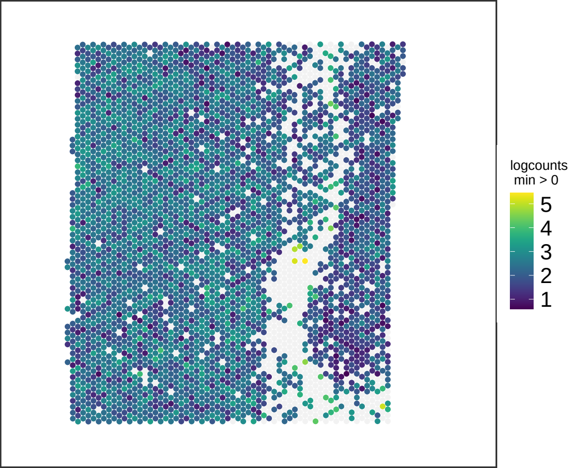
V13M06-388_C1 CAMK2N1
