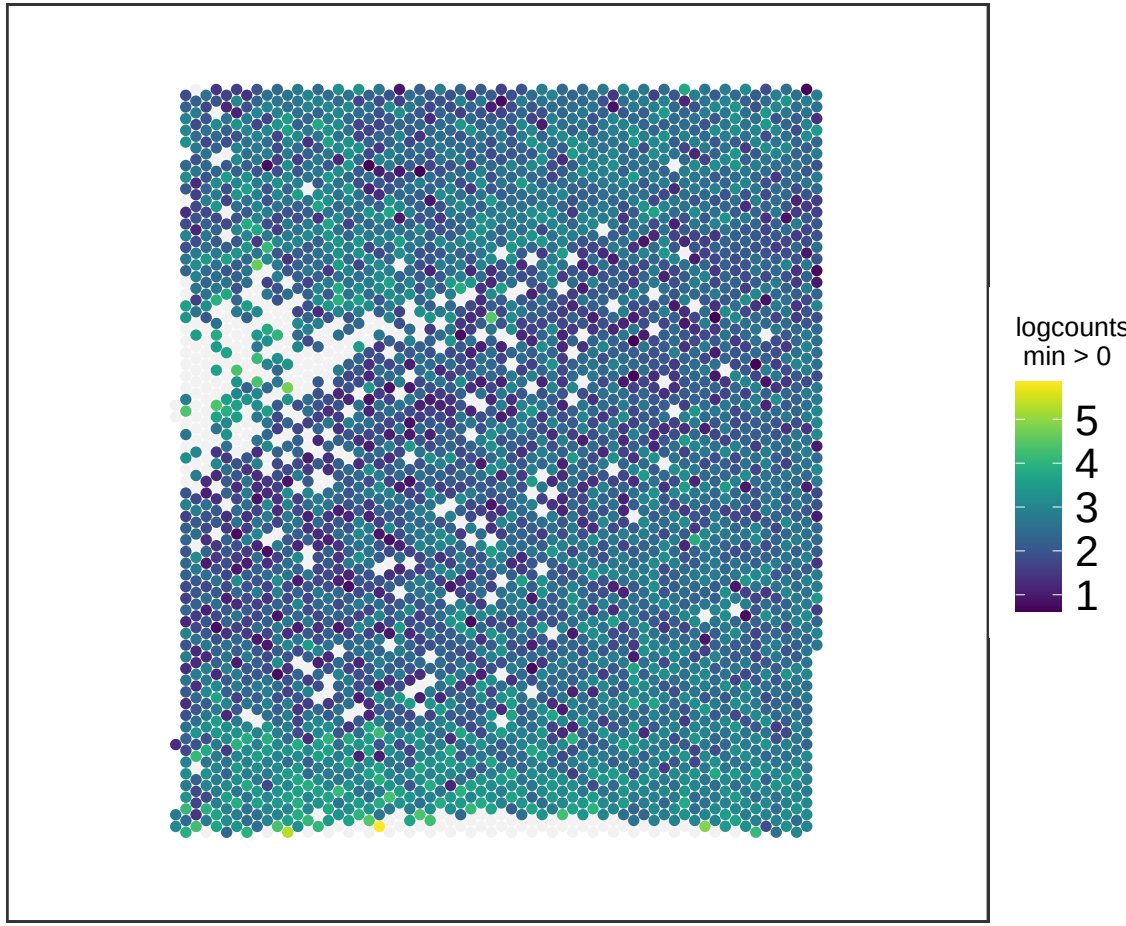
V13M06-388_D1 CAMK2N1
