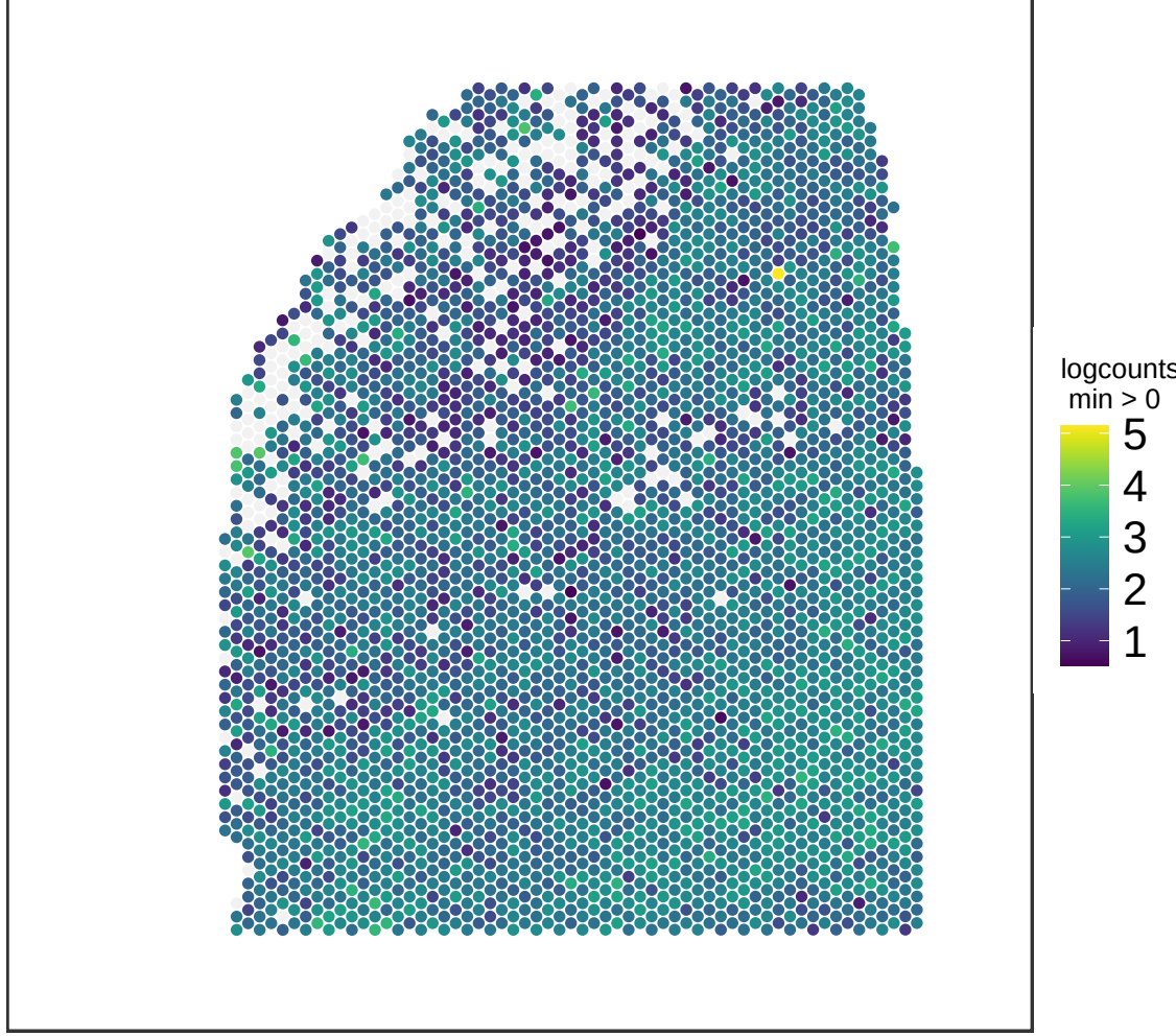
V13M06-388_B1 CAMK2N1
