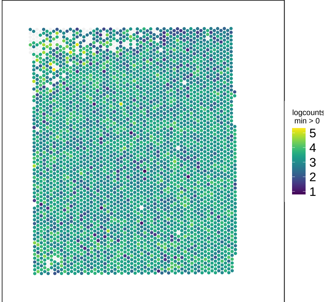
V13M06-387_B1 CAMK2N1
