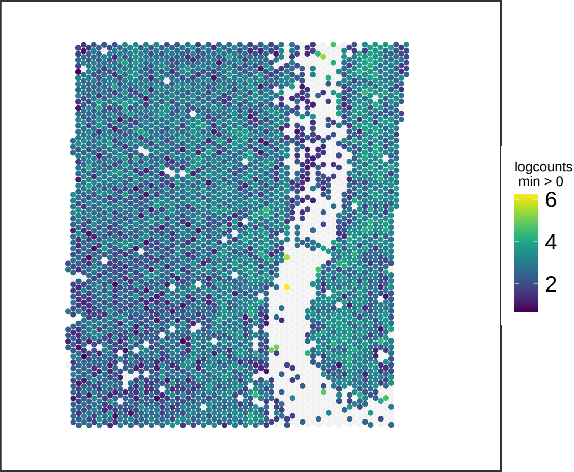
V13M06-388_C1 RTN1
