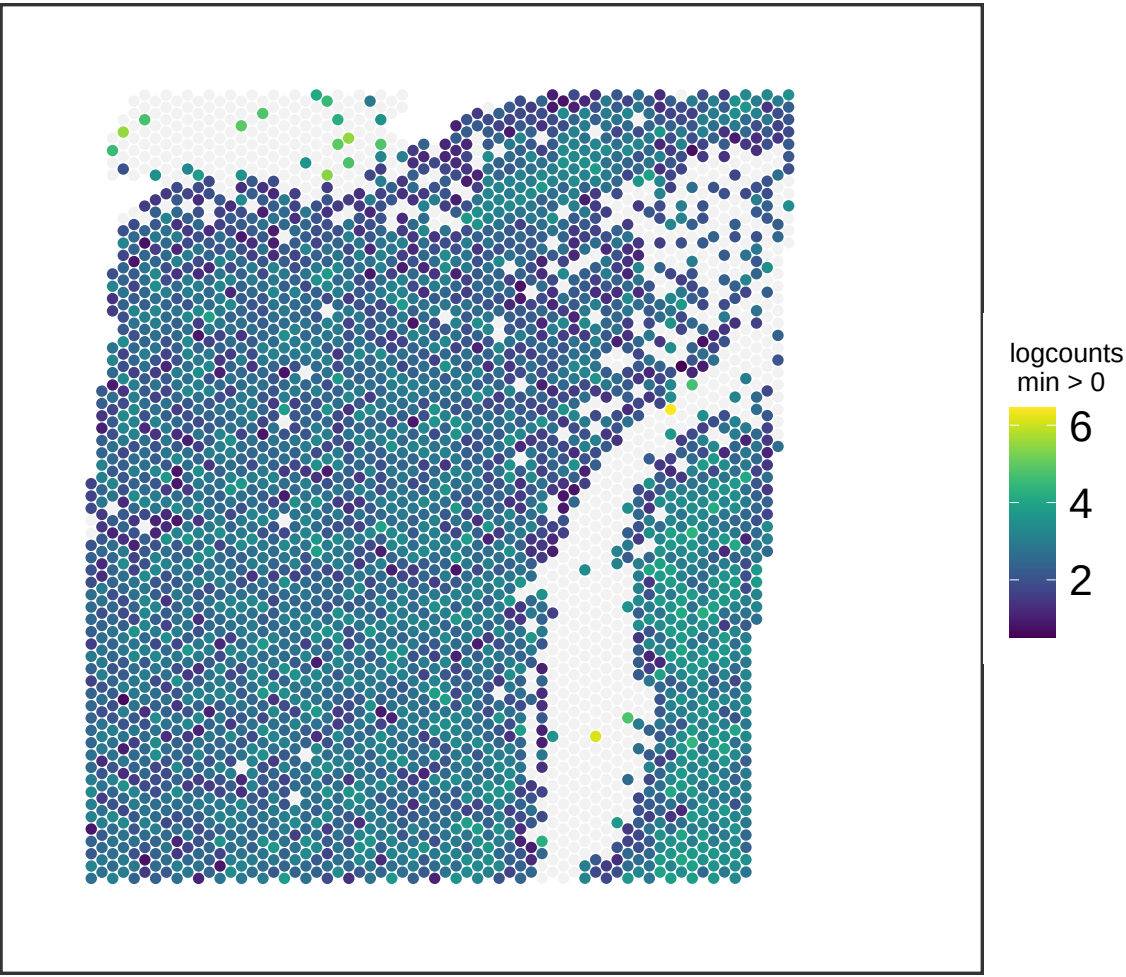
V13M06-388_A1 RTN1
