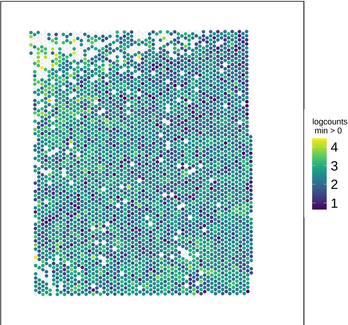
V13M06-387_B1 RTN1
