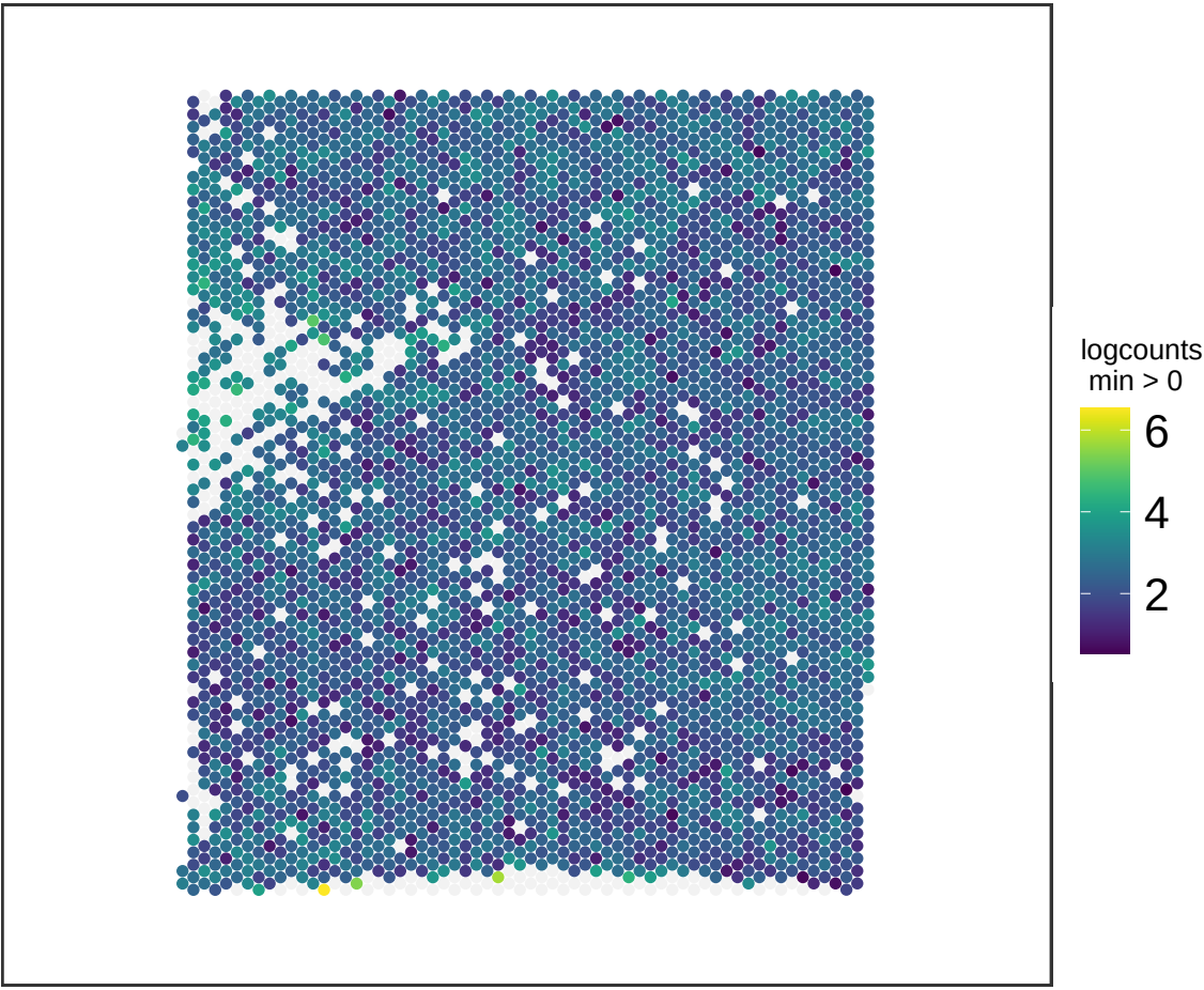
V13M06-388_D1 RTN1
