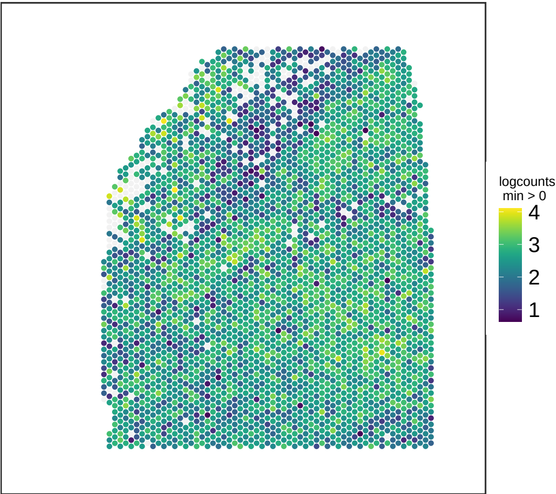
V13M06-388_B1 RTN1
