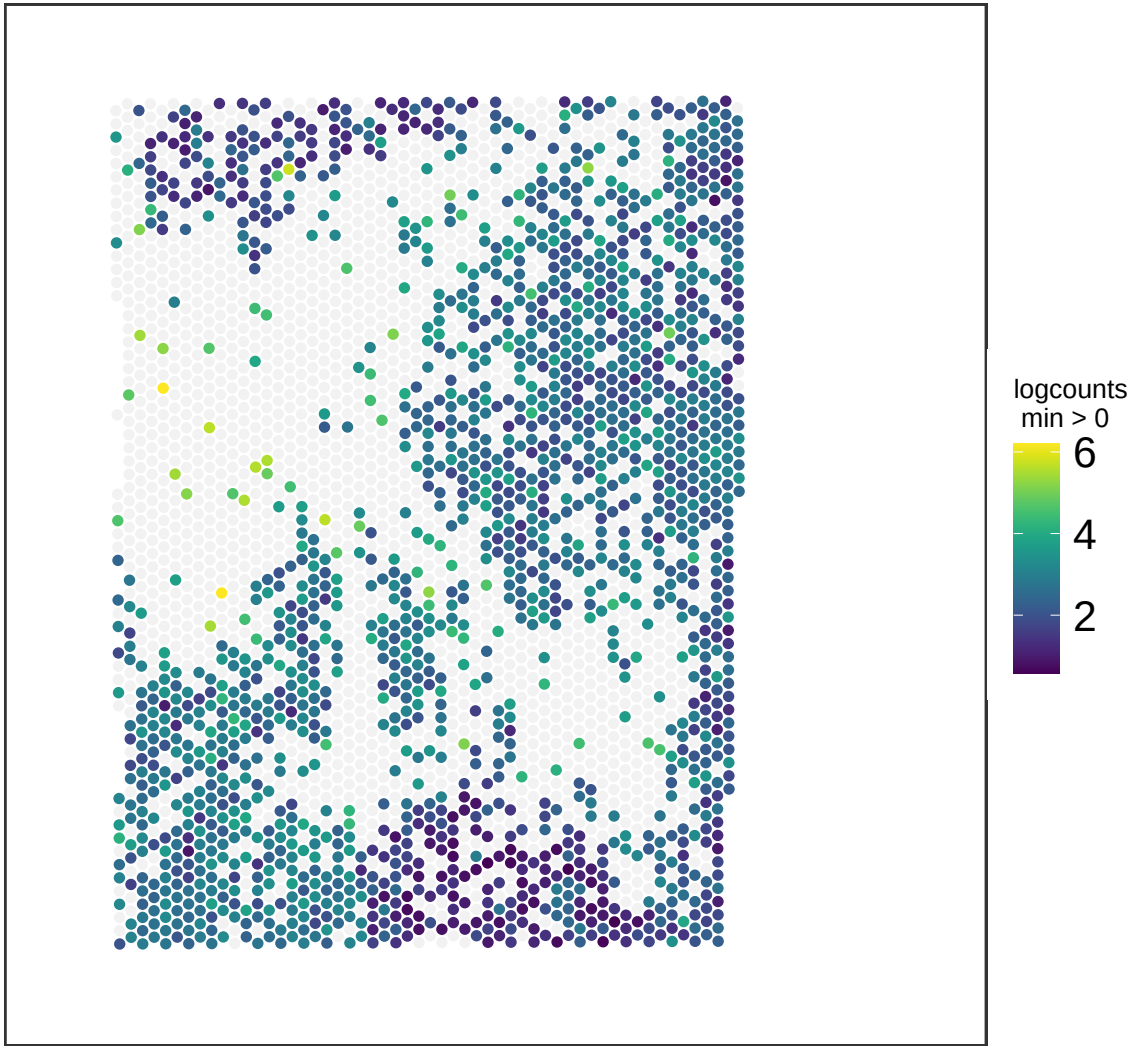
V13M06-387_C1 RTN1
