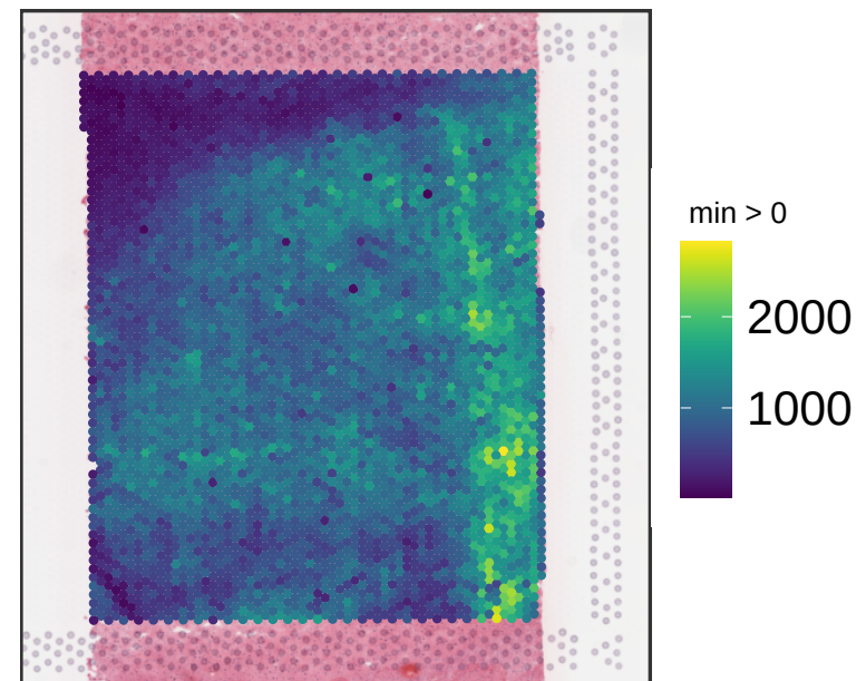
V13M06-387_B1 expr_chrV
