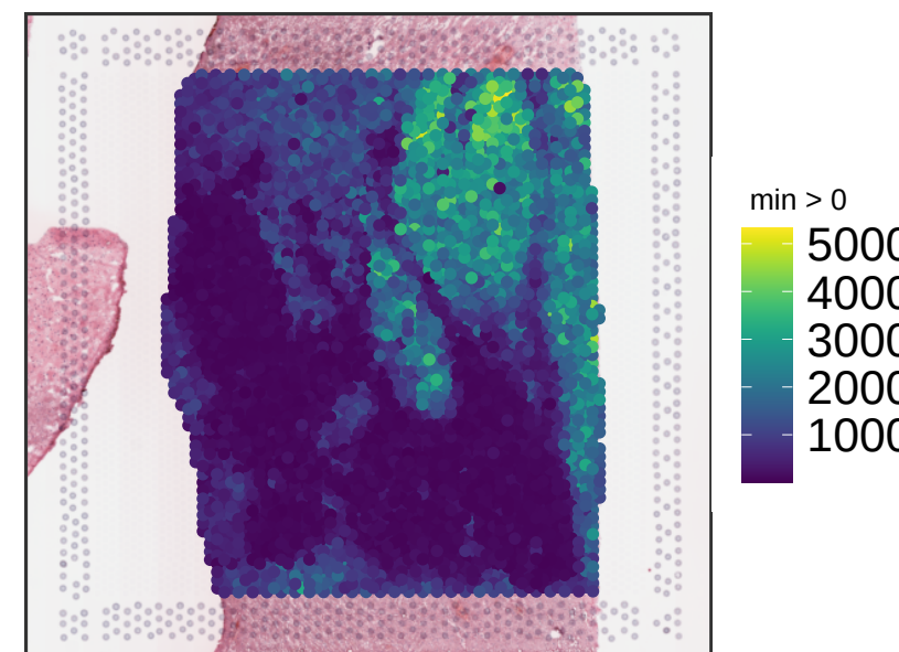
V13F27-366_B1 sum_gene
