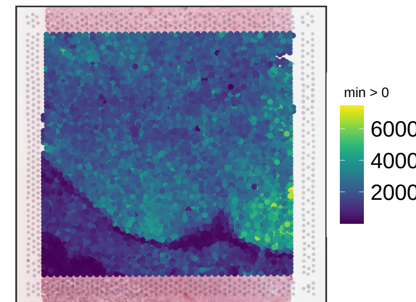
V13F27-366_C1 sum_gene
