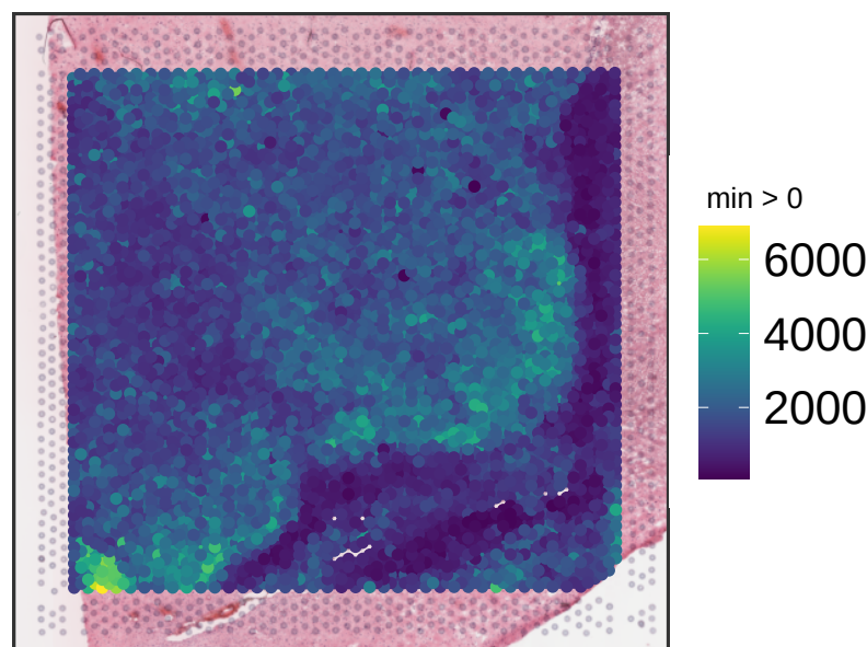
V13F27-366_A1 sum_gene
