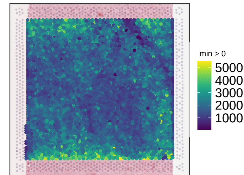
V13F27-366_D1 sum_gene
