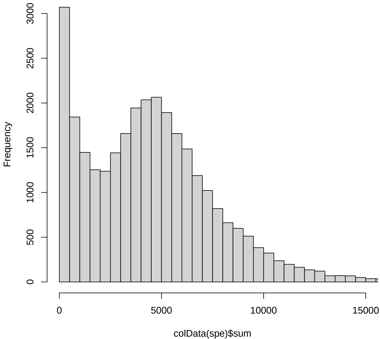
Histogram of colData(spe)$sum
