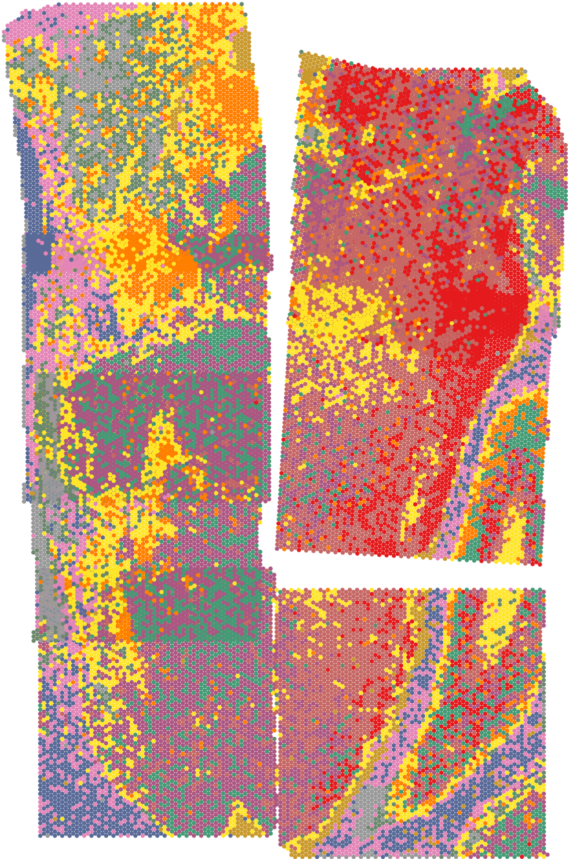
clust_HARMONY_M0_lam0.4_kmeans11
