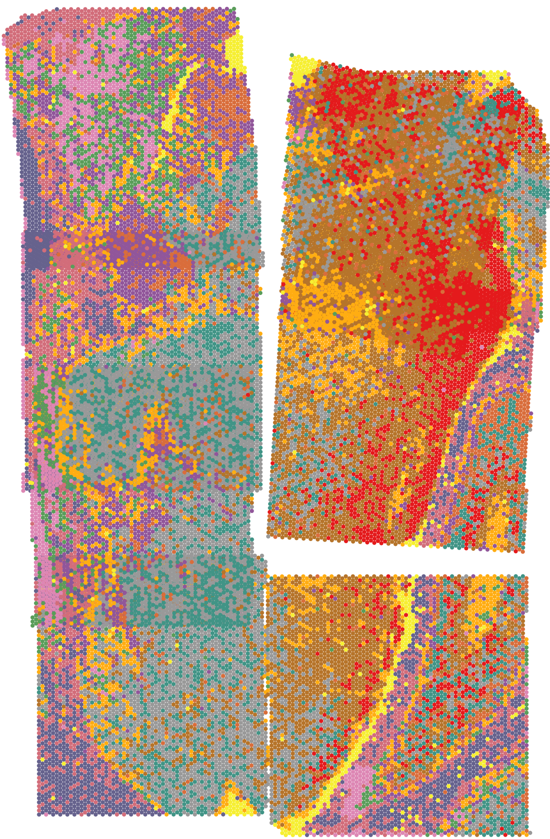
clust_HARMONY_M0_lam0.4_kmeans12
