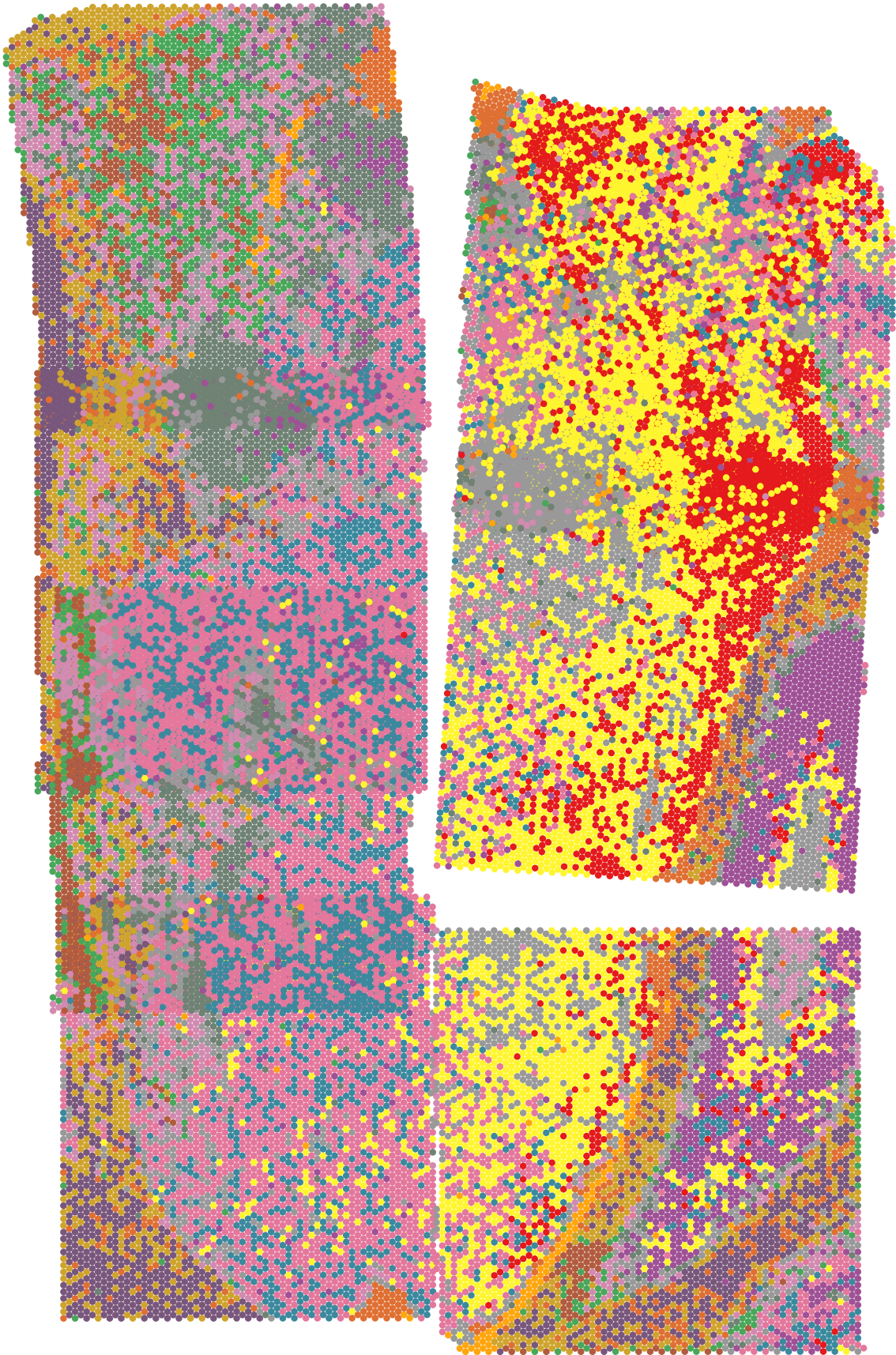
clust_HARMONY_M0_lam0.4_kmeans14
