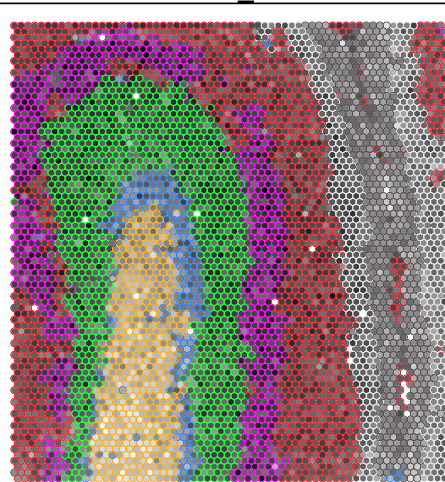
Br5973_SCZ
