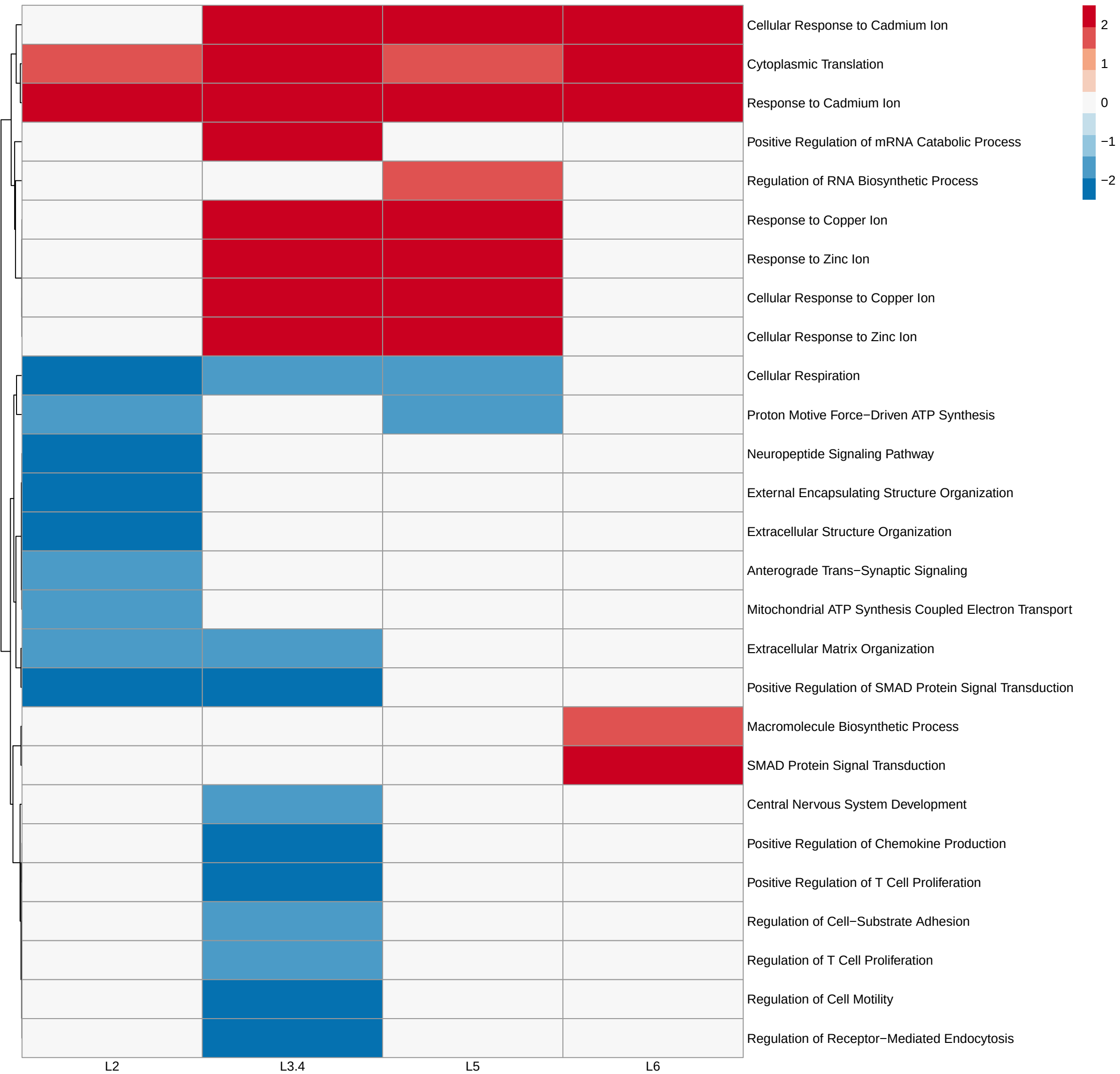
NTC.BPD F GO-BP NES of sig. terms as fill color (0 if not sig.)
