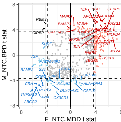
MDD females & BPD males common (vs NTC)
