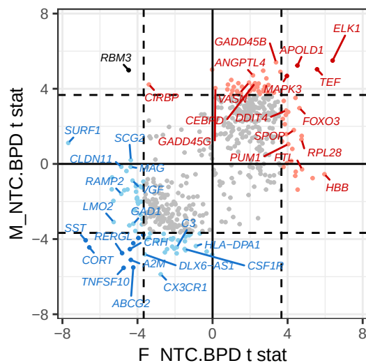
BPD females & BPD males common (vs NTC)
