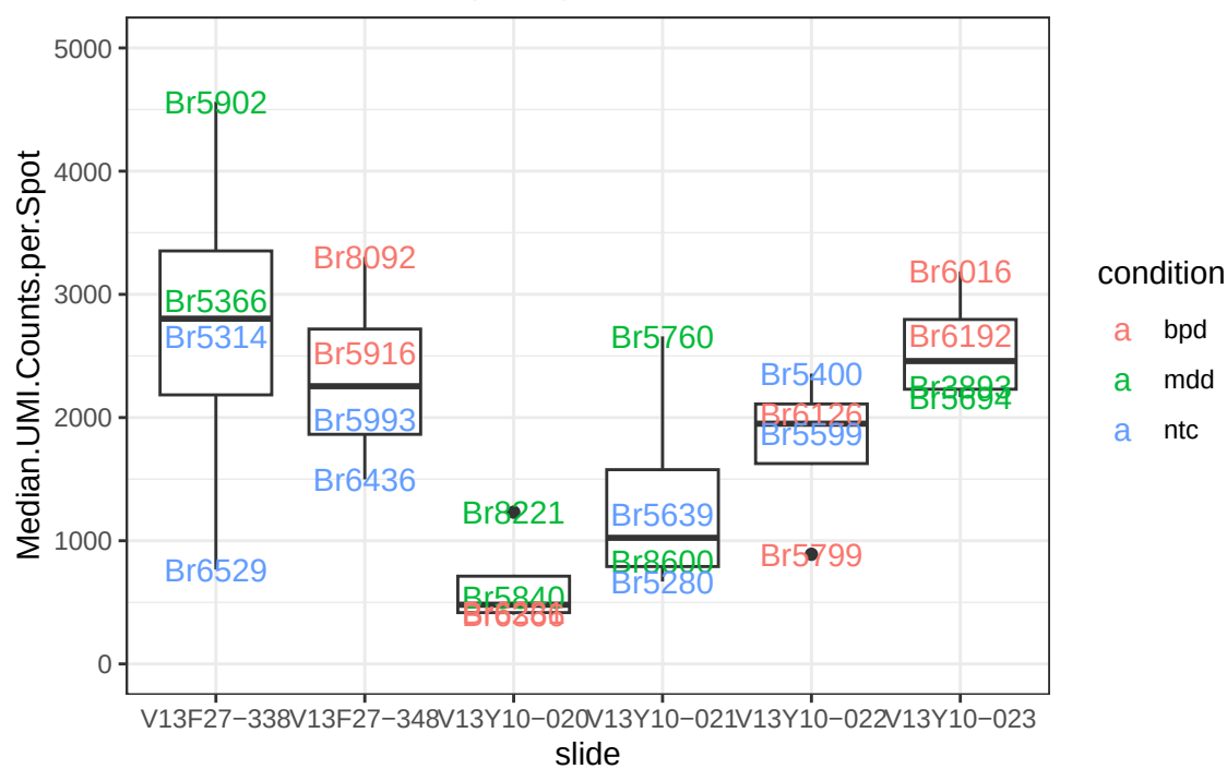
Median.UMI.Counts.per.Spot
