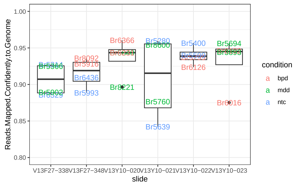
Reads.Mapped.Confidently.to.Genome
