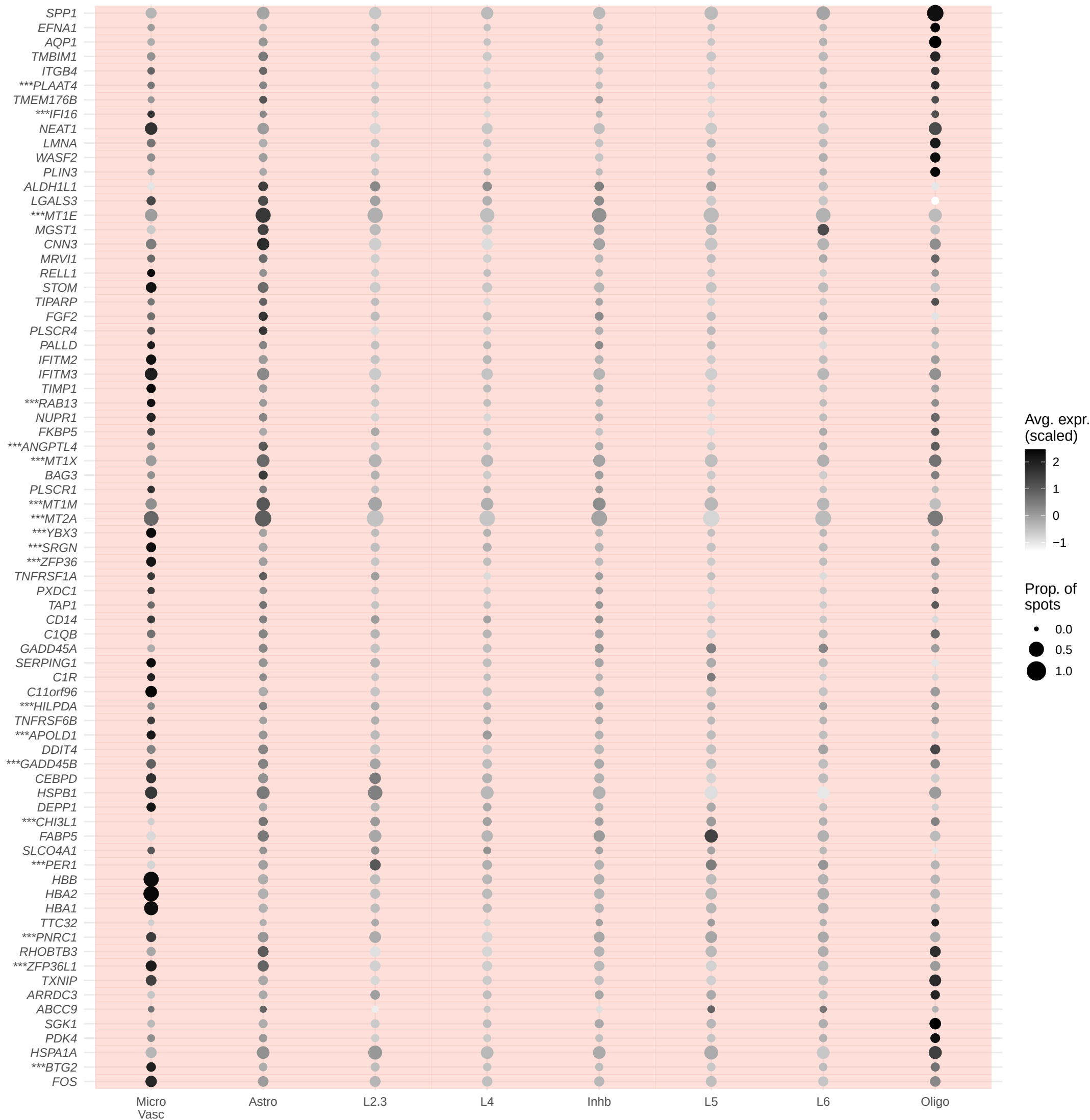
NTC.MDD F L-A DEGs with abs(logFC)>.3 and zero prop.>2% in half of capture areas (background indicates whether term was enriched/depleted)
