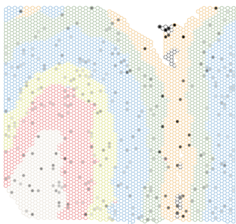
MUSTN1
