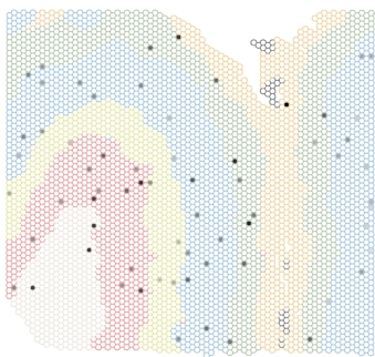
ABCG2
