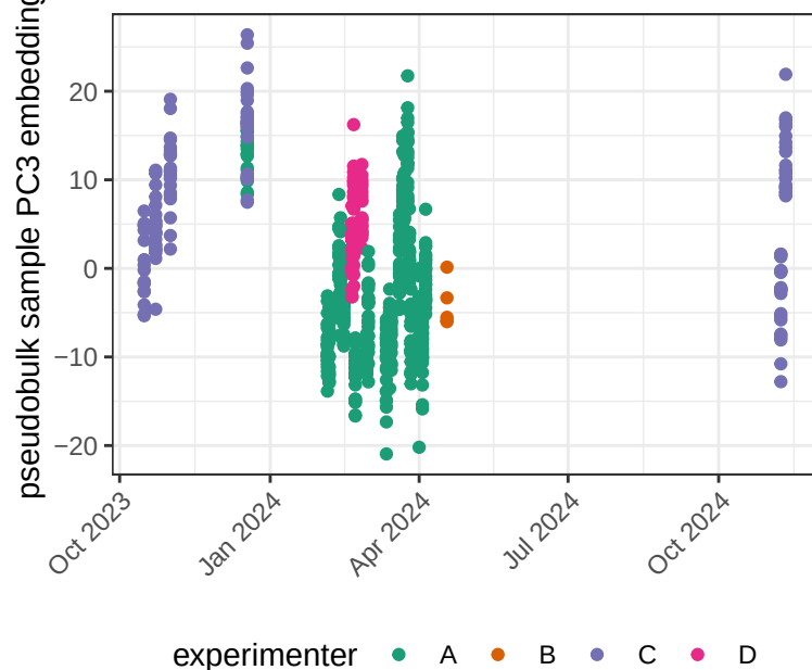
PRECAST (smoothed)
