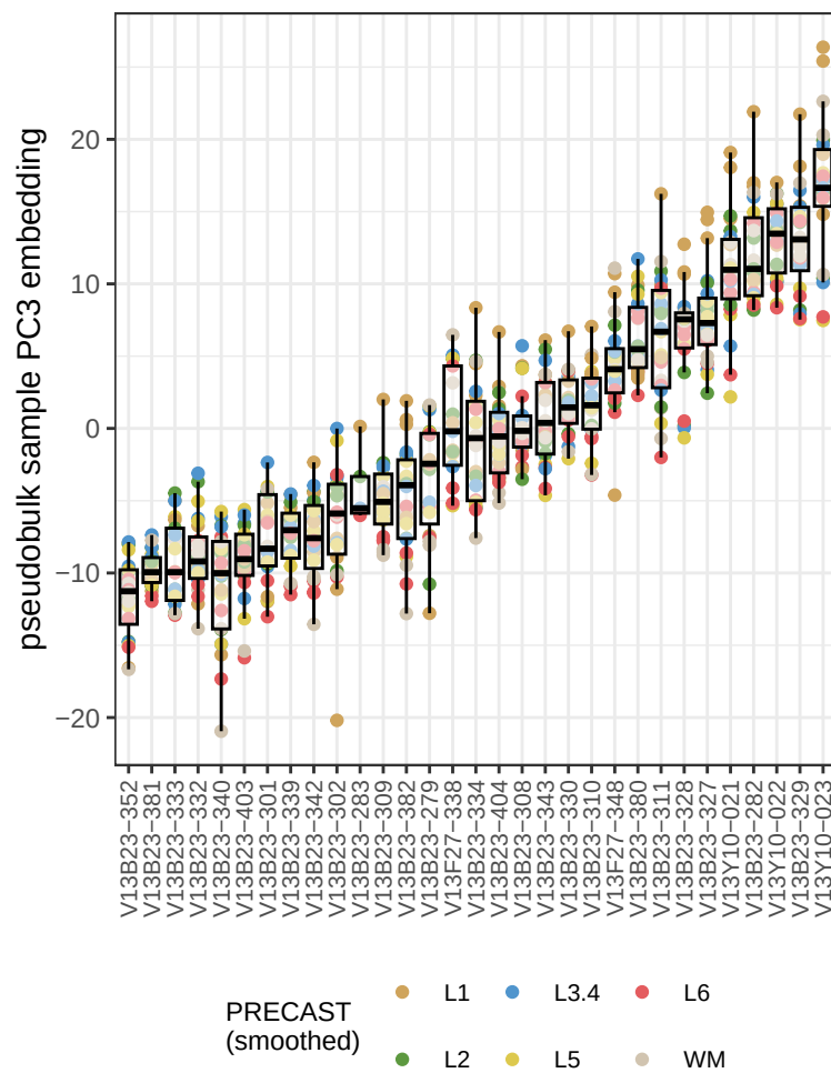
PRECAST (smoothed)
