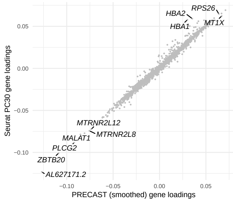
PRECAST (smoothed)
