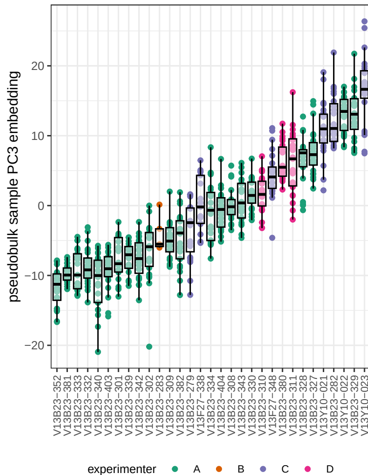
PRECAST (smoothed)
