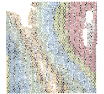
BPD M
