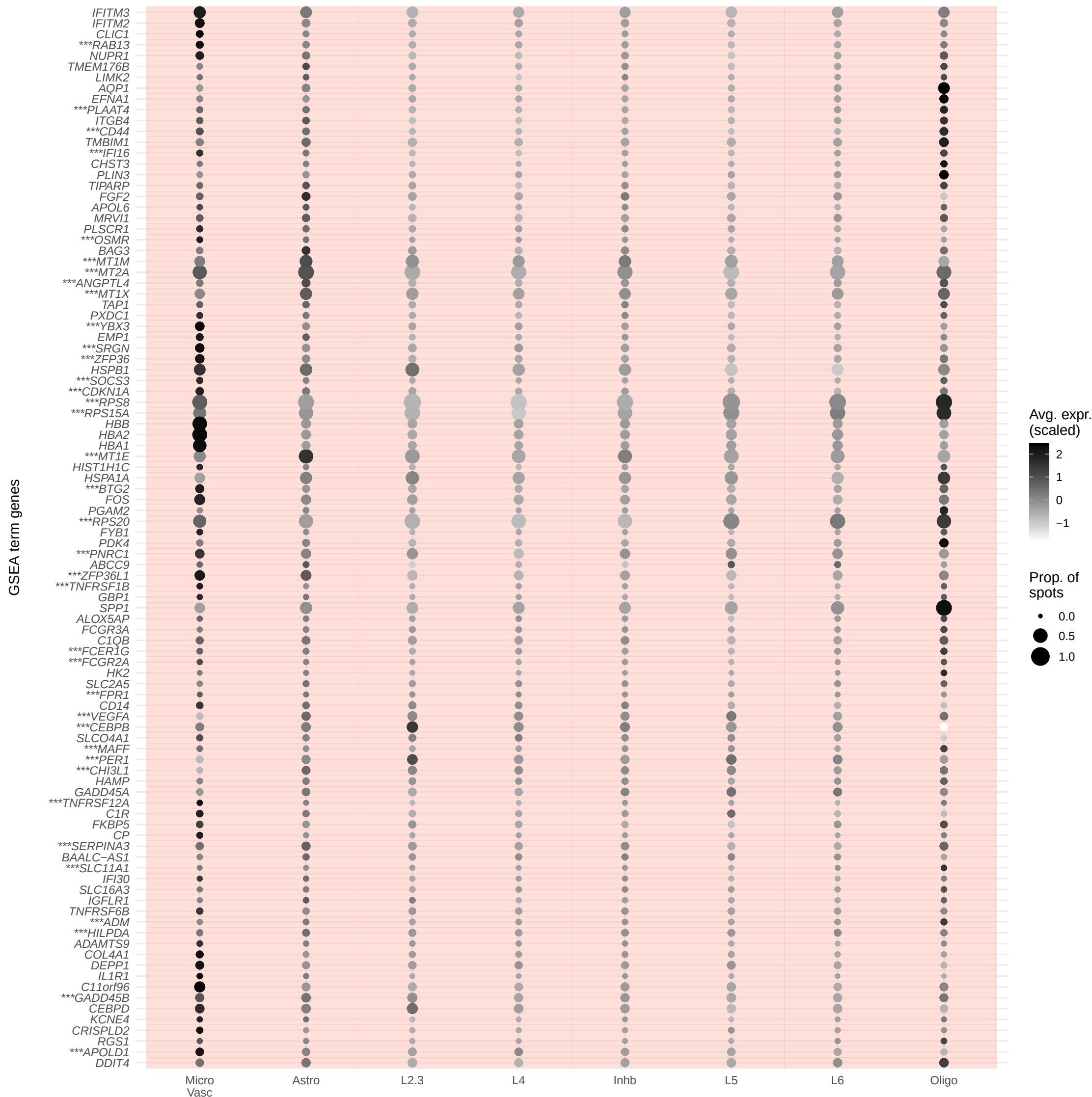
NTC.MDD F L-A DEGs with abs(logFC)>.5 (background indicates whether term was enriched/depleted)
