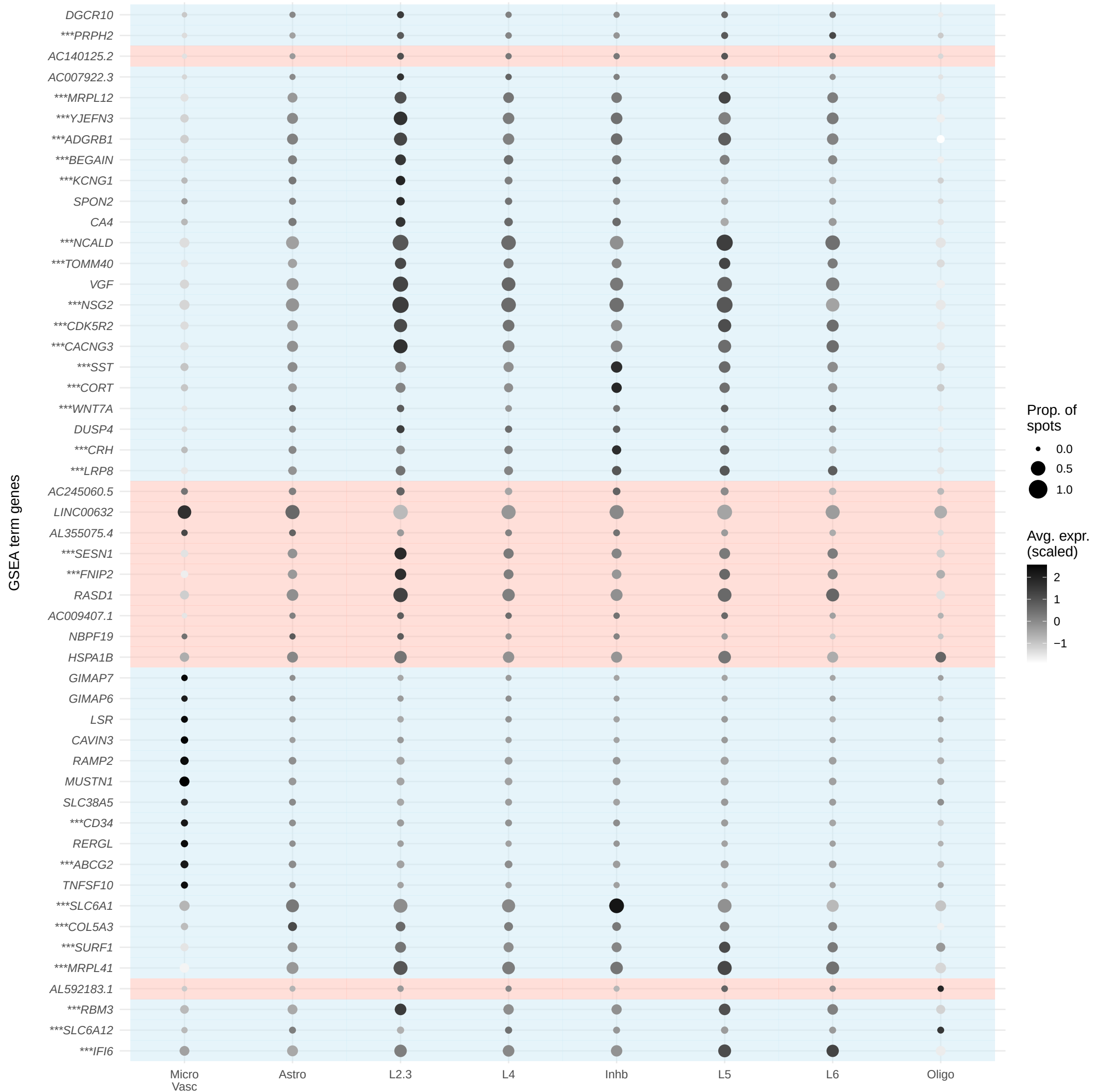
NTC.MDD F L-A DEGs with \text{abs}(\log\text{FC}) > .5 (background indicates whether term was enriched/depleted)
