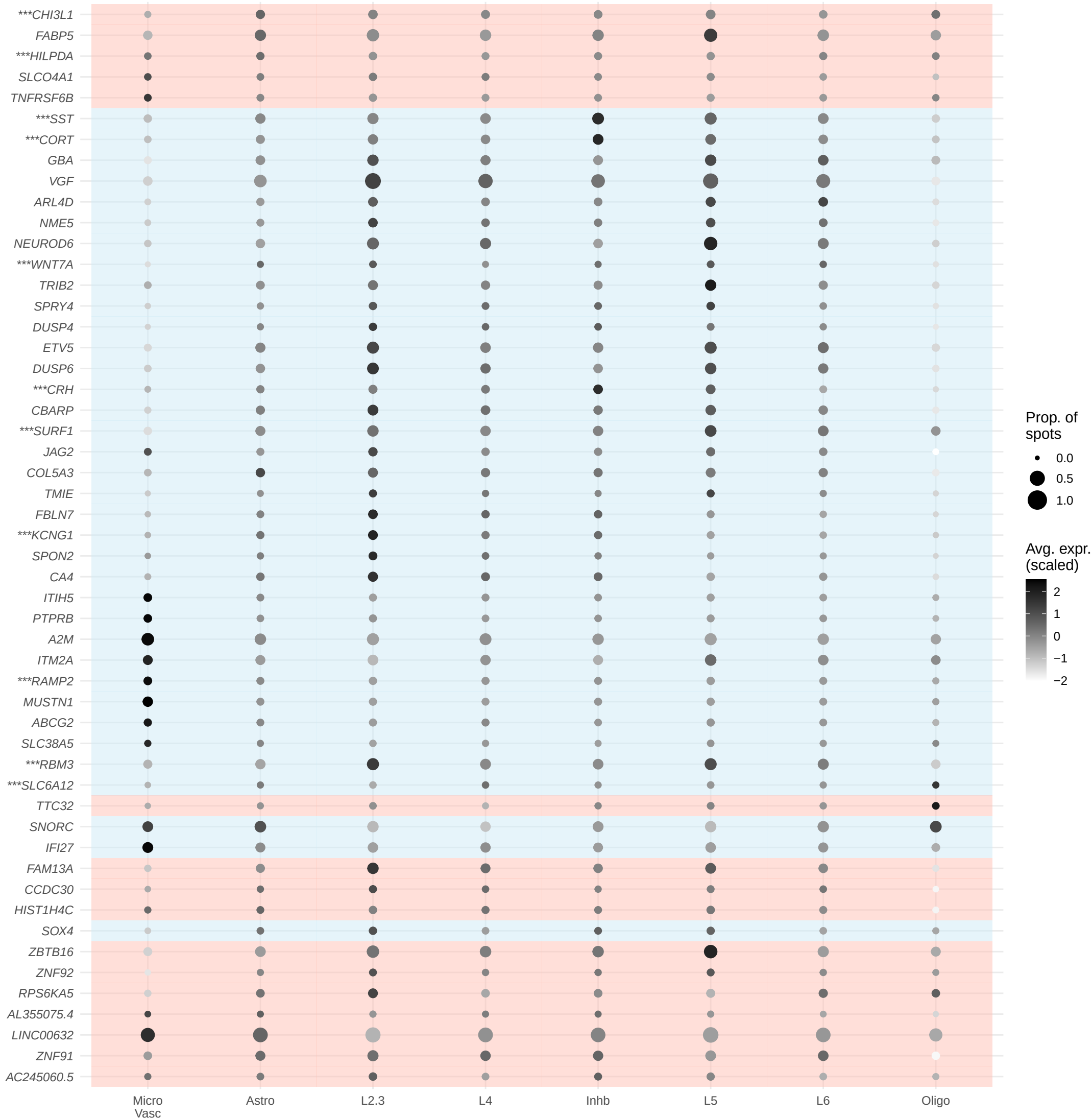
NTC.MDD F L-A DEGs with \text{abs}(\log\text{FC}) > .3 and zero prop. > 2% in half of capture areas (background indicates whether term was enriched/depleted)
