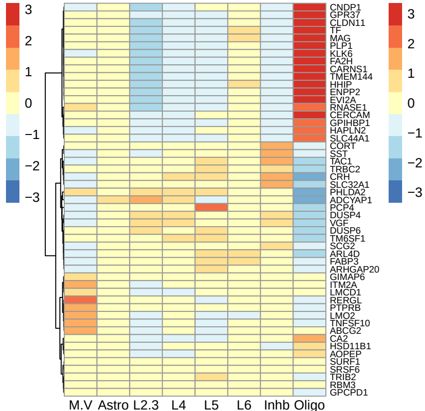
Seurat: NTC.BPD F, decreased (logcount expr heatmap)
