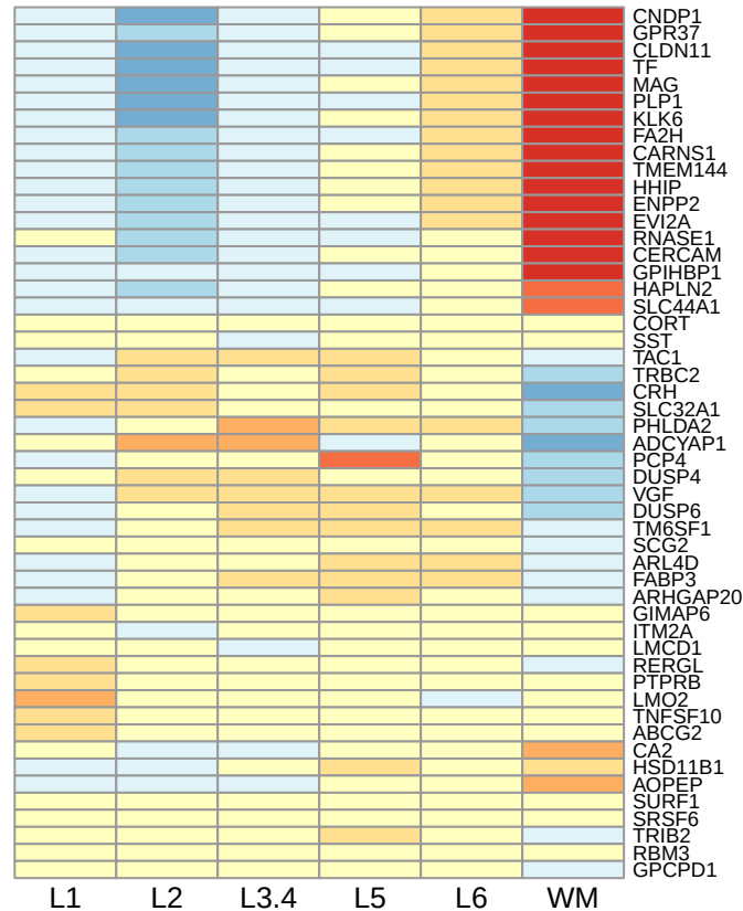
PRECAST: NTC.BPD F, decreased (logcount expr heatmap)
