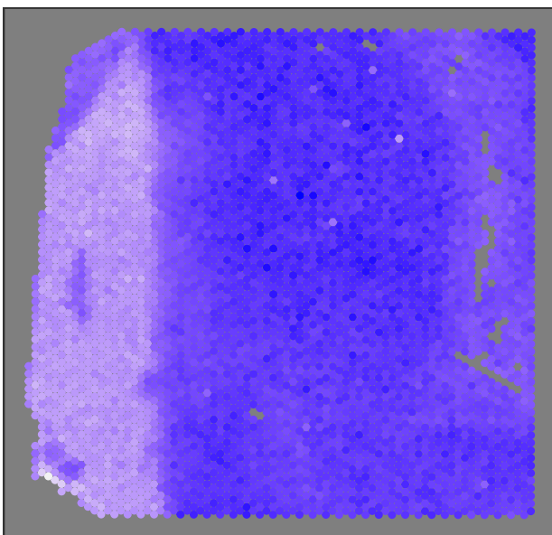
Sum UMI (log10)
