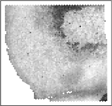
lg10.genes
