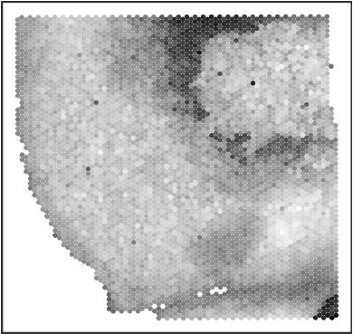
lg10.sum
