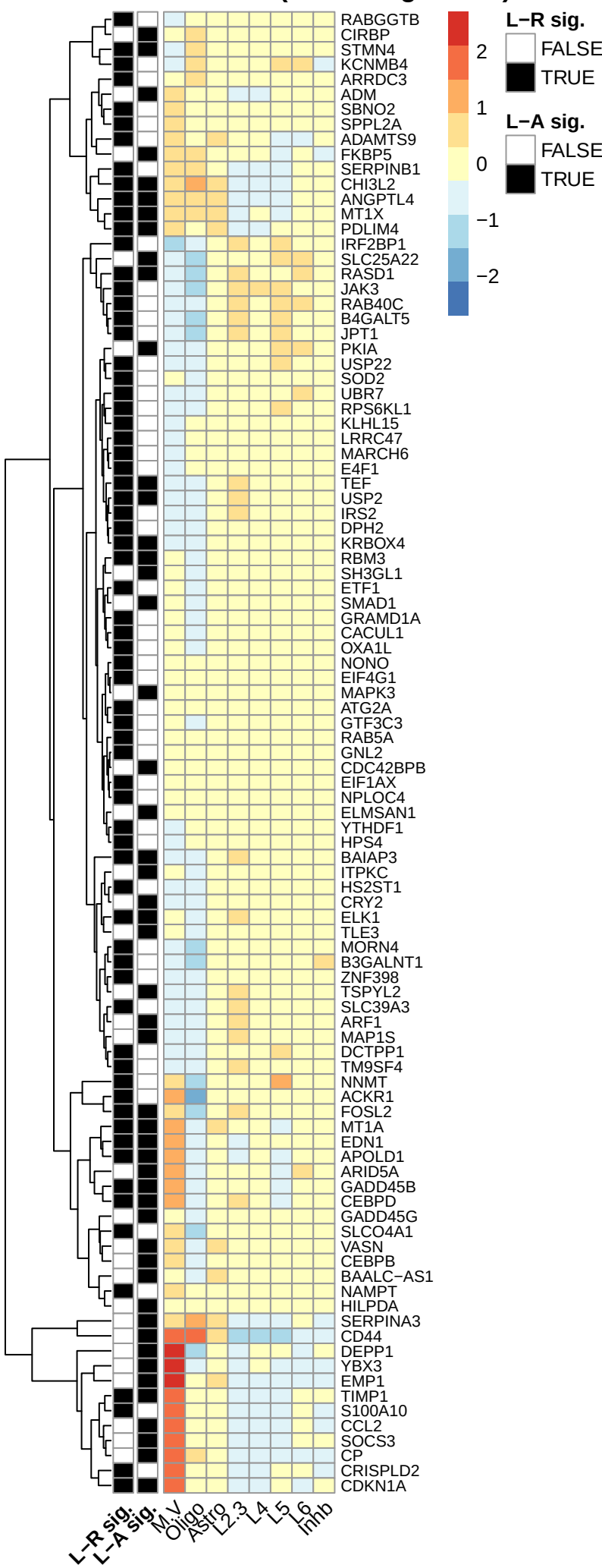
NTC.BPD M: Increased (scaled logcounts)
