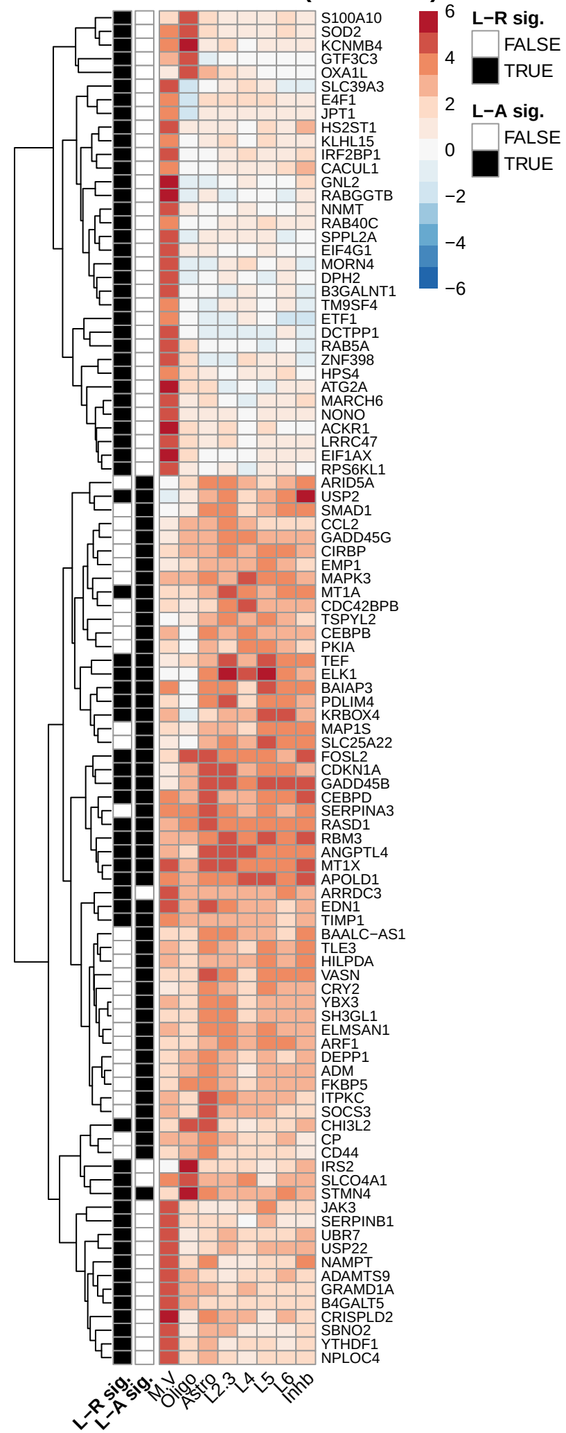
NTC.BPD M: Increased (t statistics)
