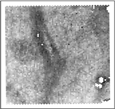
lg10.genes
