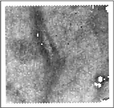
lg10.sum
