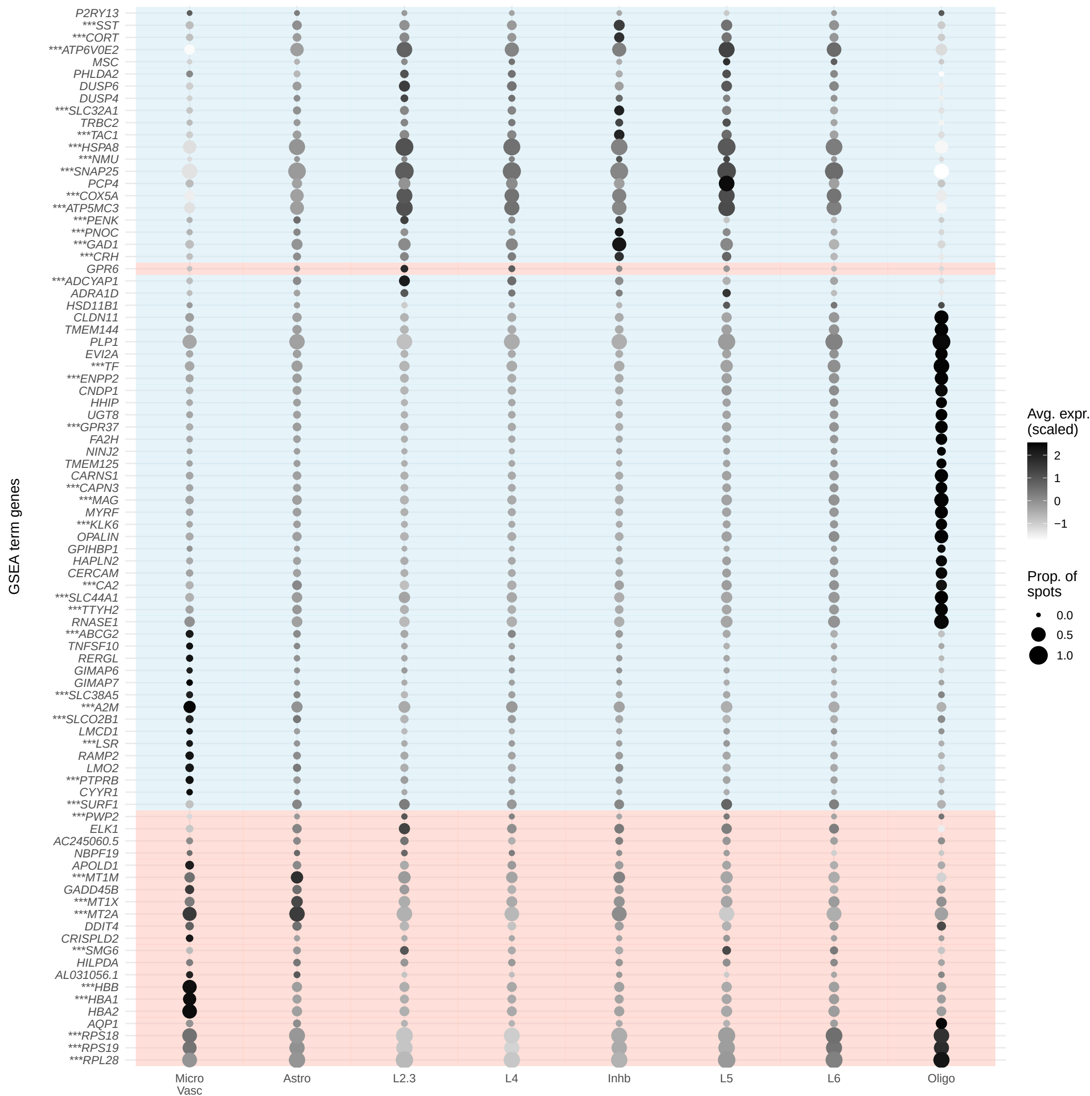
NTC.BPD F L-A DEGs with abs(logFC)>.5 (background indicates whether term was enriched/depleted)
