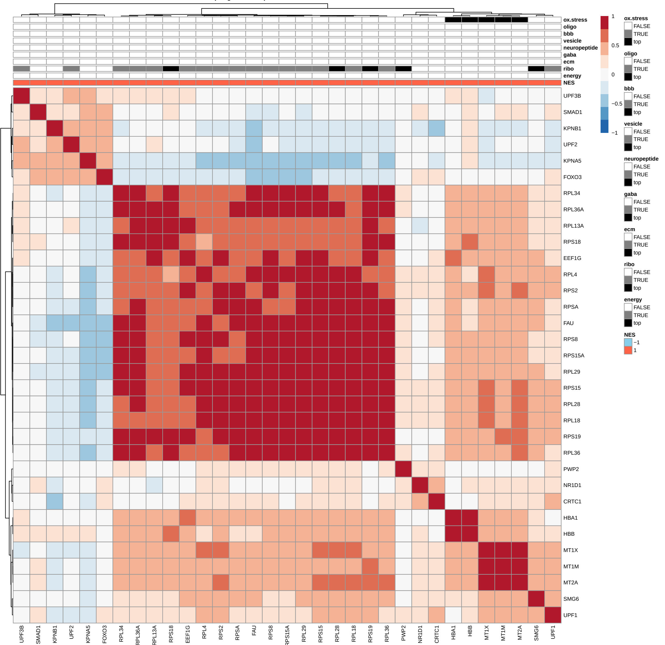
NTC.BPD F L-A enriched genes Top logFC DEGs per theme annotated with black
