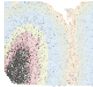
PLP1
