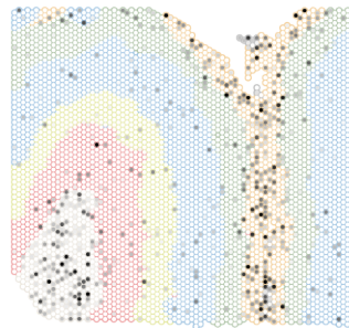
CAMK2N1
