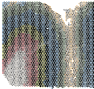
UQCRH
