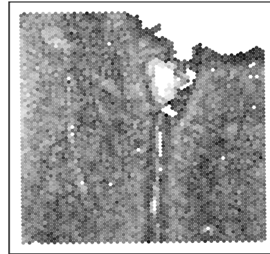
post-filt chrM ratio
