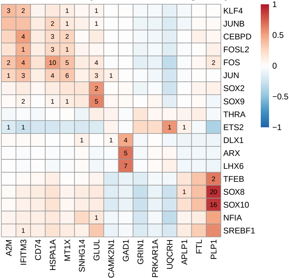
UCell correlation (DEG modules vs regulons)
