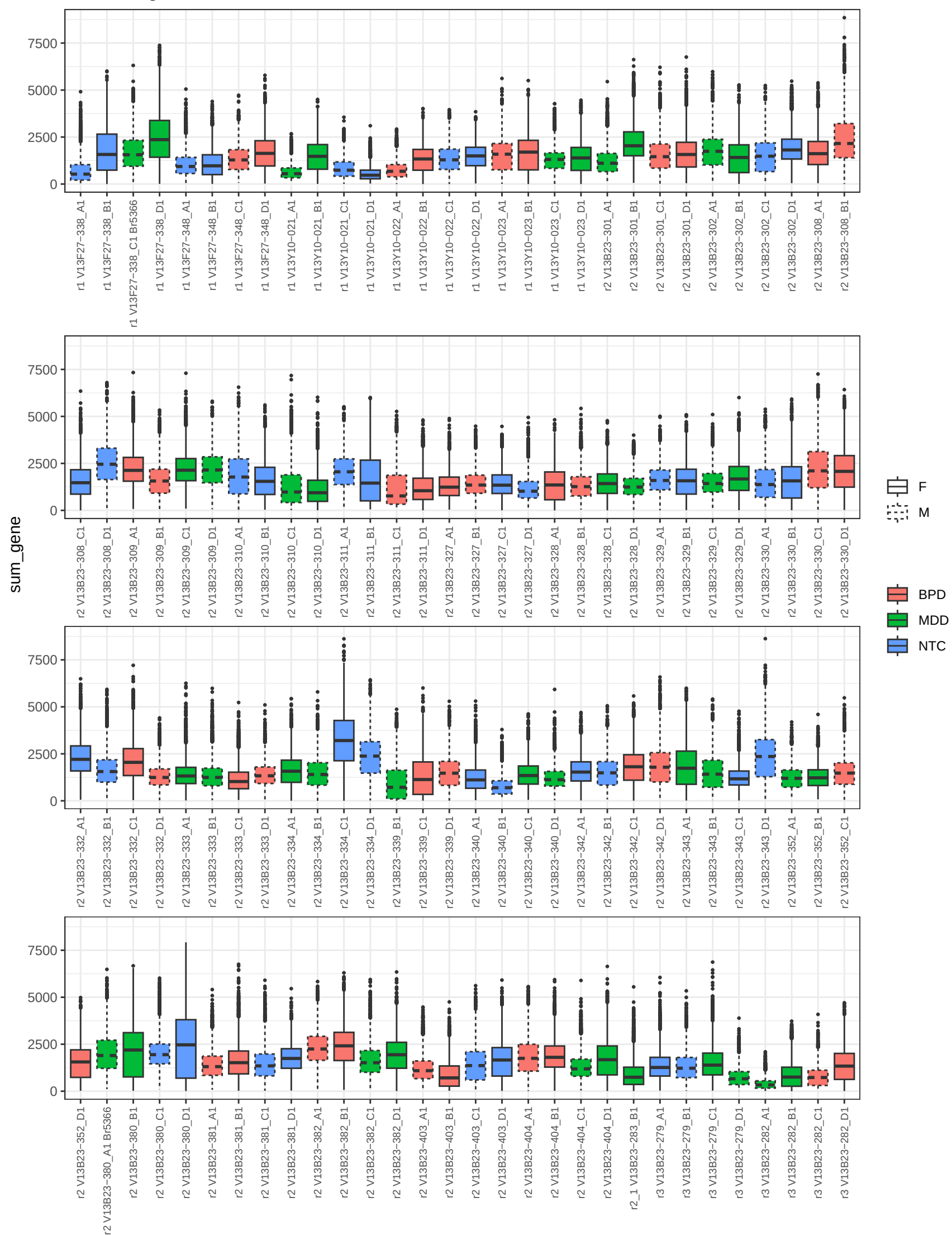
Detected genes
