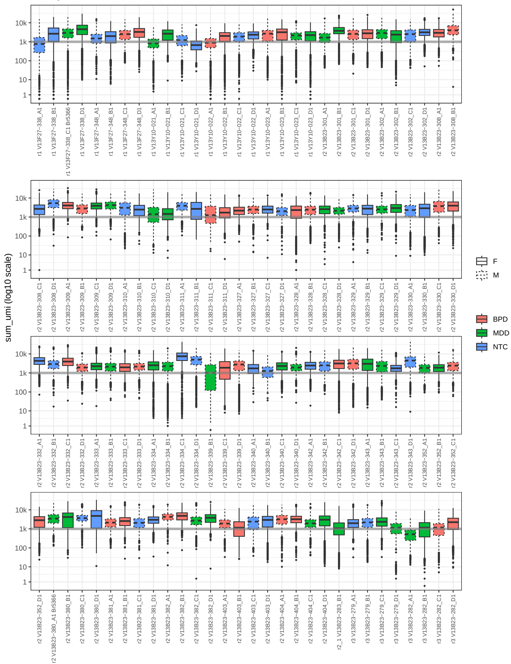
Library size
