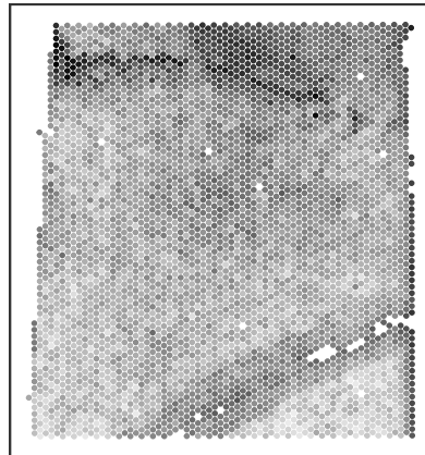
post-filt lg10(UMI counts)
