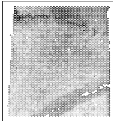
post-filt lg10(n genes)
