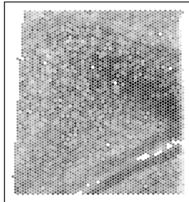
post-filt chrM ratio
