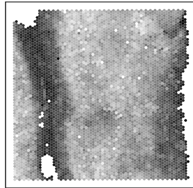
post-filt \lg_{10}(\text{UMI counts})
