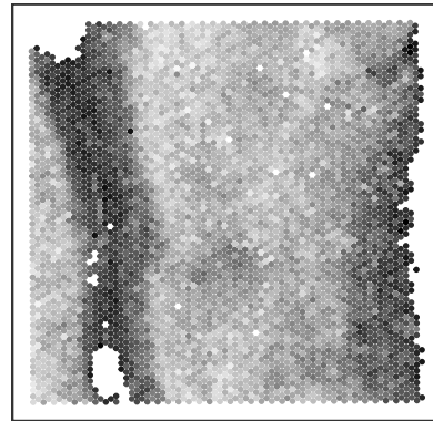
post-filt \lg_{10}(\text{n genes})
