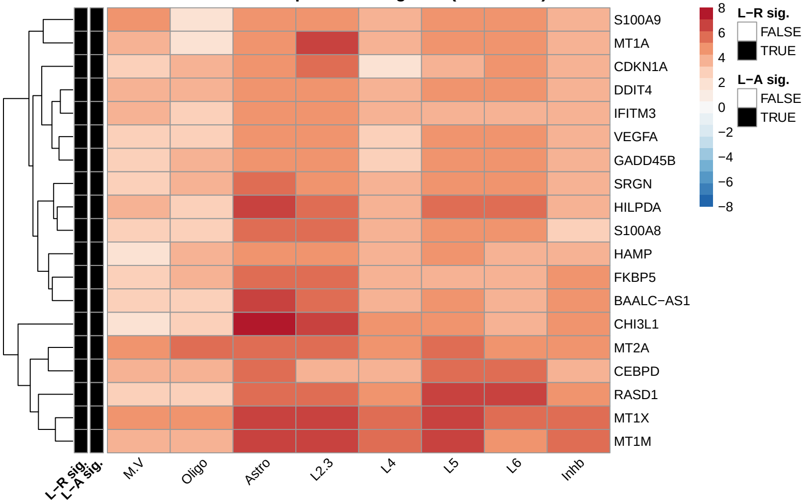
NTC.MDD F: Top increased genes (scaled logcounts)
