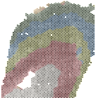
BPD M
